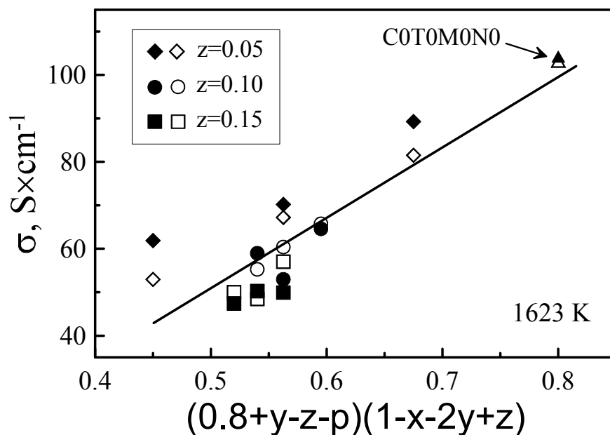
Fig. 8. Comparison of experimental conductivity data of \text{Fe}_{2.8-x-y-z-p}\text{Mg}_{0.2}\text{Cr}_x\text{Ti}_y\text{Mn}_z\text{Ni}_p\text{O}_4 spinels at 1623 K (closed symbols) and corresponding model behaviour described by Eq.6 (open symbols). The symbols denote the relative contents of Mn. The solid line shows the linear trend for experimental data.
