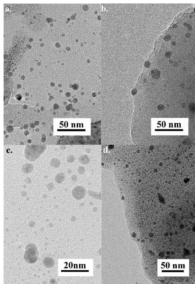
Figure 1: TEM images of a. AgNP@K Lig, b. AgNP@ K Lig/PAM, c. AgNP@TMPLig and d. AgNP@TMPLig/PAM.
