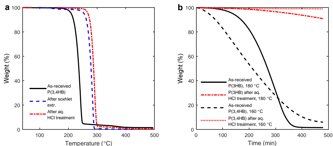
Figure 1: TGA traces of as-received and pre-treated P(3,4HB) recorded at 10 °C \text{min}^{-1} under nitrogen (a) and TGA traces showing the isothermal decomposition of P(3,4HB) and P(3HB) materials under air during 8 h at 160 and 180 °C, respectively (b).
