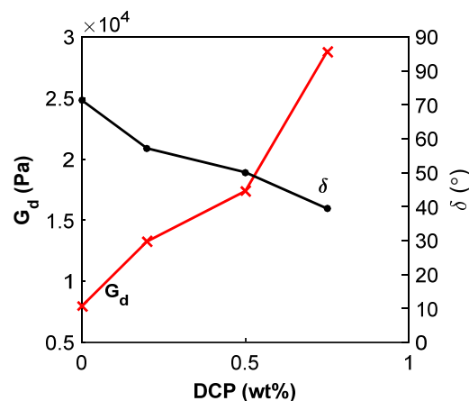
Figure 11: Dynamic shear modulus and phase shift for P(3HB):PBAT 20:80 blends with addition of DCP measured by rheology at 1 Hz and 180 °C.
