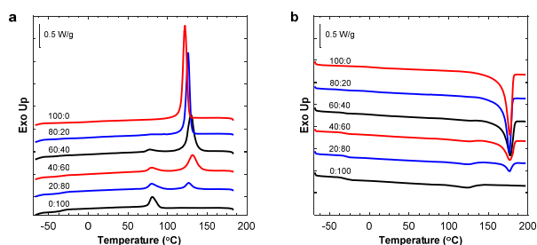
Figure 5: DSC traces of the P(3HB):PBAT blends: cooling (a) and second heating scans (b).
