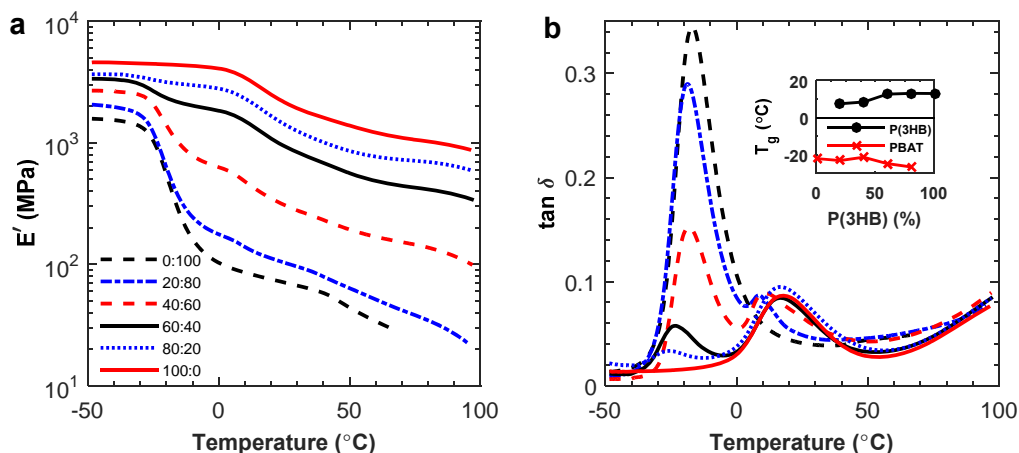
Figure 7: Tensile storage modulus (a) and \tan \delta (b) of the P(3HB):PBAT blends. The inset presents the T_g of P(3HB) and PBAT in the blends determined from the position of the loss modulus peak.
