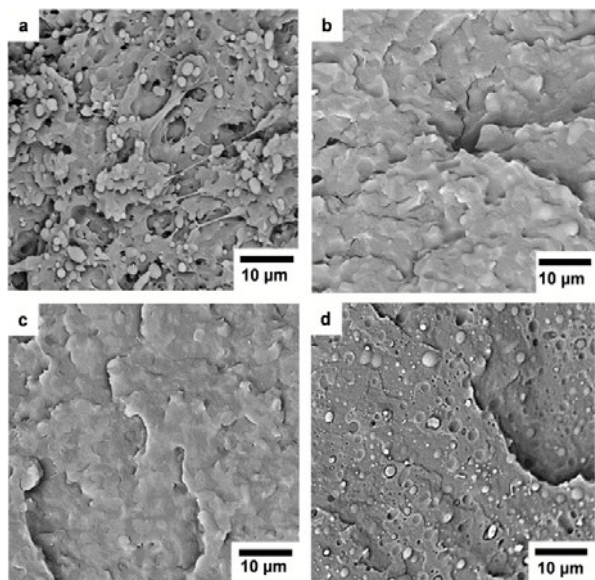
Figure 3: SEM images of cryo fractured surfaces of P(3HB):PBAT blends with (a) 20:80, (b) 40:60, (c) 60:40 and (d) 80:20 weight ratios.
