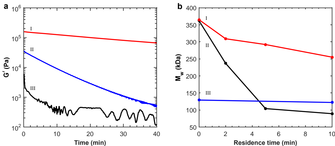
Figure 2: Degradation observed by (a) monitoring the melt shear storage modulus of P(3,4HB): (I) treated with aq. HCl solution, (II) soxhlet extracted with \text{CHCl}_3 and (III) as-received, and by (b) following the molecular weight measured by SEC of (I) HCl-treated P(3,4HB), (II) as-received P(3,4HB) and (III) PBAT.
