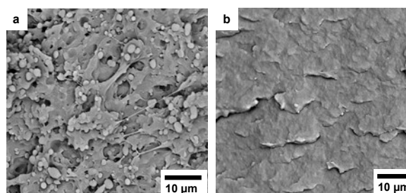
Figure 8: SEM images of cryo-fractured surfaces of P(3HB):PBAT 20:80 blends (a) without DCP and (b) with 0.5 wt% DCP added.
