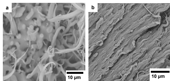
Figure 9: SEM images of room temperature fractured surfaces of P(3HB):PBAT 60:40 blends (a) without DCP and (b) with 0.5 wt% DCP added.
