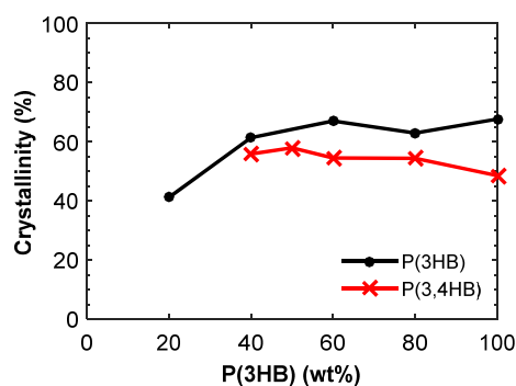
Figure 4: Crystallinity of the PHA fraction of the blends calculated from the second DSC heating scans.
