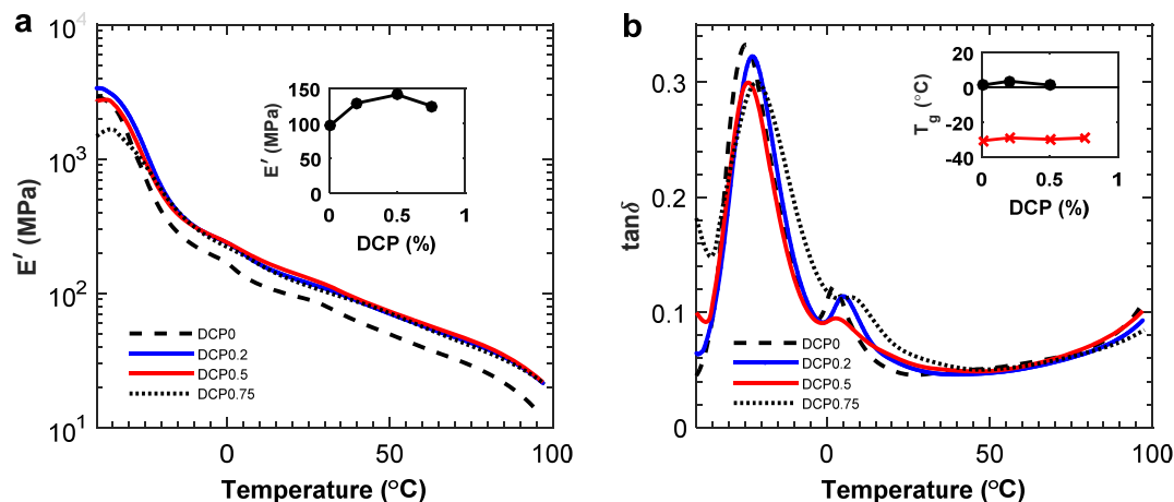
Figure 12: Tensile storage modulus (a) and \tan \delta (b) for P(3HB):PBAT 20:80 blends with addition of DCP. The inset in part (a) shows the change in E' with the content of DCP, and the inset in part (b) shows the T_g of P(3HB) (●) and PBAT (×) determined from the loss modulus peak value.
