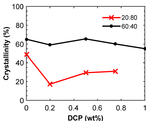
Figure 10: Crystallinity of the P(3HB) component in P(3HB):PBAT blends as a function of the DCP content. The data was calculated from the second DSC heating scans (SI, Figures S11 and S12).
