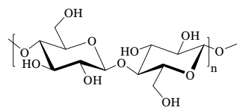
Scheme 1. The structural repeat unit in cellulose.
