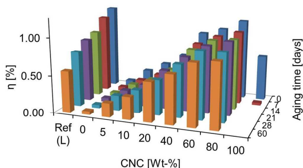
Fig. 5. DSSC efficiency, \eta , as a function of CNC content and aging time. The results depicted are average values of duplicate cells.
