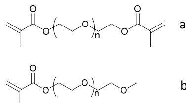
Scheme 3. Structures of the PEO oligomers used in the study; (a) PEODMA and (b) PEOMA.
