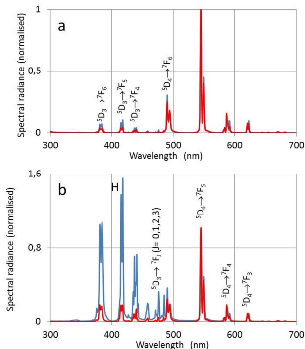
Fig. 8 Emission spectra of (\text{Y}_{1-x}\text{Gd}_x)_2\text{O}_2\text{S}:\text{Tb}^{3+} for x = 0 (blue) and x = 1 (red) and 2 mol% \text{Tb}^{3+} excited at 270 nm (a) and for 0.1 mol% \text{Tb}^{3+} (b). H in (b) indicates the normalised maximum spectral radiance of the ^5\text{D}_3 \rightarrow ^7\text{F}_5 transition.
