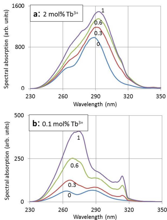
Fig. 4 PL excitation spectra of (Y_{1-x}Gd_x)_2O_2S:Tb^{3+} ( x = 0, 0.3, 0.6 and 1 ) calcined at 900 °C and monitored at 545 nm with 2 mol% Tb^{3+} (a) and with 0.1 mol% Tb^{3+} (b).
