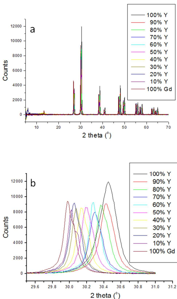
Fig. 1 (a) XRPD pattern of the 2 mol% Tb^{3+} ( Y_{1-x}Gd_x ) _2O_2S:Tb^{3+} phosphor family calcined at 900 °C. (b) Enlarged view of the main peak around 30° (2 \theta ).
