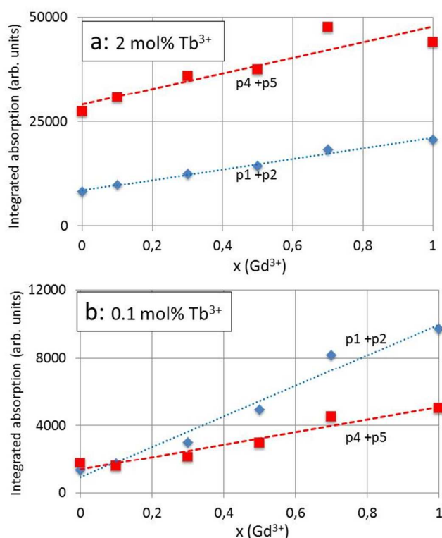
Fig. 7 Integrated absorption of CT-band components of (\text{Y}_{1-x}\text{Gd}_x)_2\text{O}_2\text{S}:\text{Tb}^{3+} (calcined at 900 °C) monitored at 545 nm with 2 mol% \text{Tb}^{3+} (a) and with 0.1 mol% \text{Tb}^{3+} (b). Dashed curves (polynomials) in (b) have been fitted to the experimental points.
