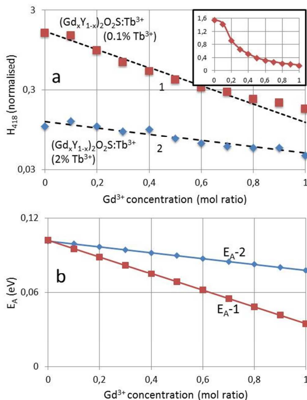
Fig. 11 (a): Normalised amplitude of {}^5D_3 \rightarrow {}^7F_5 transition at 418 nm versus Gd^{3+} concentration. Points are experimental values; the dashed lines are calculated with Eq. (3). (b): E_A for the two Tb^{3+} series, no. 1 for 0.1 mol% Tb^{3+} and no. 2 for 2 mol% Tb^{3+} are indicated as a function of x . E_{A-1} and E_{A-2} are expressed in eV. The insert of (a) is a linear plot of H_{418} (line 1) versus Gd^{3+} concentration.
