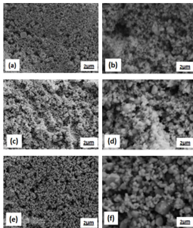
Fig. 3 (a & b) Y_2O_2S:Tb^{3+} phosphor particles 2% Tb^{3+} , 900 °C, (c & d) Y_{0.50}Gd_{0.50}O_2S:Tb^{3+} phosphor particles 2% Tb^{3+} , 900 °C, and (e & f) Gd_2O_2S:Tb^{3+} phosphor particles 2% Tb^{3+} , 1100 °C. Magnification (a, c, & e) 20 kX and (b, d & f) 100 kX.
