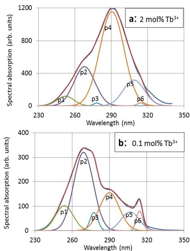
Fig. 5 Deconvolution of excitation spectrum of (Y_{1-x}Gd_x)_2O_2S:Tb^{3+} with x = 0.7 and 2 mol% Tb^{3+} (a) and with x = 0.7 and 0.1 mol% Tb^{3+} (b) with six Gaussian profiles.
