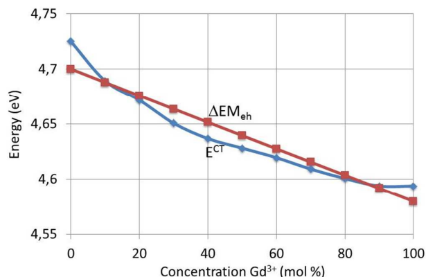
Fig. 14 E^{\text{CT}} (experimental data) and \Delta\text{EM}_{\text{eh}} as a function of \text{Gd}^{3+} concentration for (\text{Y}_{1-x}\text{Gd}_x)_2\text{O}_2\text{S}:\text{Tb}^{3+} .
