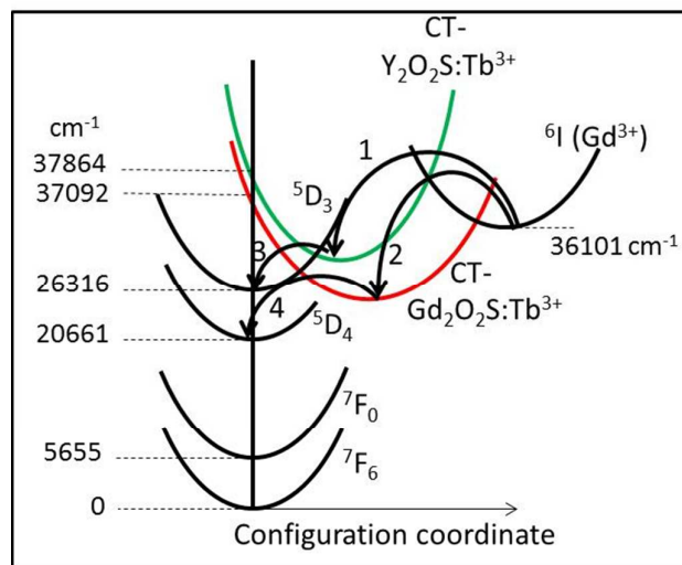
Fig. 12 Configuration diagram of Y_2O_2S:Tb^{3+} and Gd_2O_2S:Tb^{3+} . Configuration coordinates of CT-levels of Y_2O_2S:Tb^{3+} , Gd_2O_2S:Tb^{3+} and {}^6I Gd^{3+} levels are different. Arrows 1, 2, 3 and 4 indicate radiationless energy transfer.
