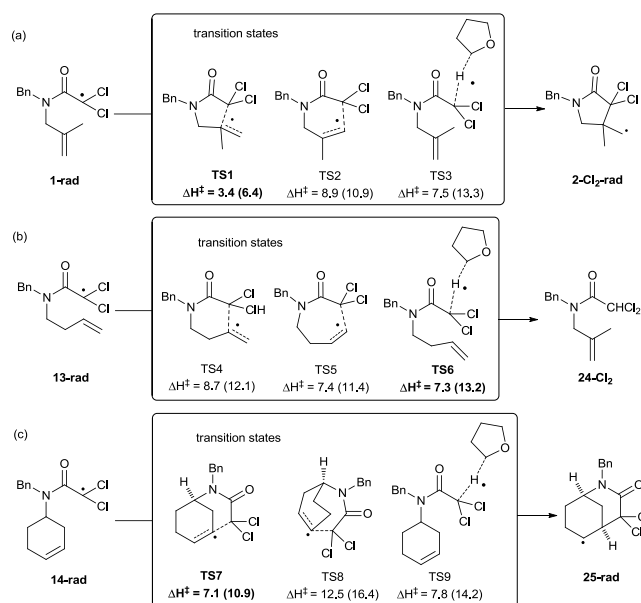
Scheme 4. Enthalpy values computed for the transition states arising from 1-rad , 13-rad , and 14-rad at M06-2X/6-311+G(d,p) level of theory. Values in parenthesis correspond to B3LYP/6-311+G(d,p).
