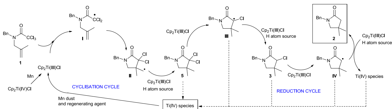
Scheme 3. Proposed mechanism for titanocene(III)-catalysed radical cyclisation of trichloroacetamides.
