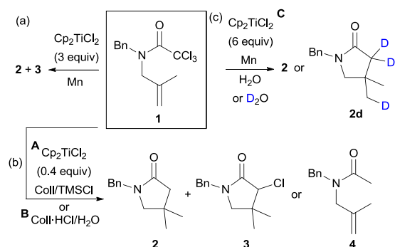
Scheme 2. \text{Cp}_2\text{TiCl} -mediated/catalysed cyclisations of trichloroacetamide 1 .
