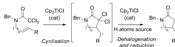
Scheme 1. Proposed \text{Cp}_2\text{TiCl} -catalysed radical cyclisation of trichloroacetamides.
