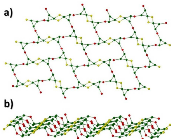
Figure 4 (a) Connectivity schematic taken from the crystal data of 2 illustrating its [3,6] net topology. Colour code: Green (Cr), Yellow (Na) and Red (O). Note: The yellow and red spheres represent Na1 and O15 (hydronium ion), respectively. (b) A single 2D sheet observed in 2 .
