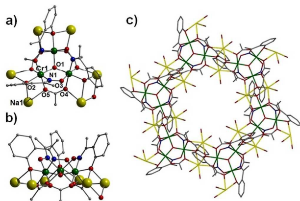
Figure 8 A single \{\text{Cr(III)}_3\text{O}\}^{7+} unit along with the linker \text{Na}^+ ions (yellow spheres) as viewed perpendicular (a) and parallel (b) to the triangular plane in 5 . (c) An array of six \{\text{Cr(III)}_3\text{O}(\text{O}_2\text{CCH}_3)_3(\text{Me-sao})_3\}^{2-} units linked by \text{Na}^+ ions to form the hexagonal [3,6] honeycomb topology in 5 .
