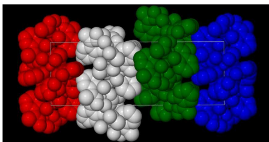
Figure 10 Space-fill representation of the parallel stacking of the individual (colour coded) 2D [6,3] nets in 5 , highlighting their staggered arrangements with respect to one another. All MeCN solvent molecules and H atoms have been omitted for clarity.
