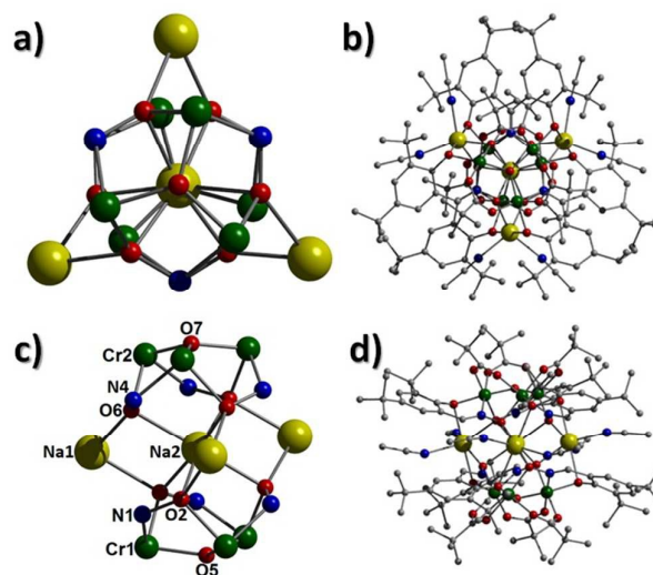
Figure 5 Inorganic core (left) and complete cage (right) in 3 , as viewed perpendicular (a and b) and parallel (c and d) to the {Cr(III) 3 O(O 2 CC(CH 3 ) 3 ) 3 (3,5-di- t Bu-sao) 3 } 2- triangular units.
