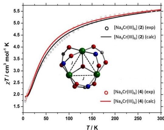
Figure 11 \chi T (per [\text{Cr}(\text{III})_3] triangle) versus T for polycrystalline samples of 2 and 4 taken in the T = 300\text{--}5 \text{ K} temperature range in an applied field of B = 0.1 \text{ T} . The solid lines are a fit of the experimental data to spin-Hamiltonian (1).
