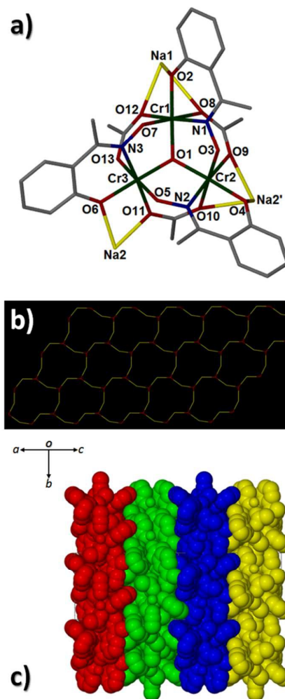
Figure 7 (a) A single {Cr(III) 3 O(O 2 CCH 3 ) 3 (Me-sao) 3 } 2- node surrounded by three connecting Na + ions as viewed perpendicular to the {Cr(III) 3 O} 7+ plane in 4 . (b) The 2D [3,6] network in 4 where the red vertices represent the O (O1) atom at the centre of the {Cr 3 O} 7+ triangular nodes and the yellow vertices represent the bridging Na + ions (Na1-2). (c) Colour coded and space-fill represented 2D nets in the unit cell of 4 .
