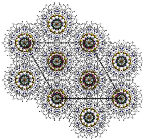
Figure 6 Crystal structure of the hexagonal packing arrangement in 3 as viewed along the c axis of the unit cell. Hydrogen atoms have been omitted for clarity.
