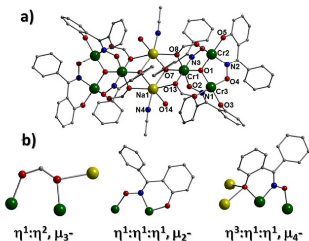
Figure 3 (a) Crystal structure of 2 minus all hydrogen atoms. (b) Selection of bonding modes exhibited by the formate (left) and Ph-sao 2- (middle and right) ligands in 2 .
