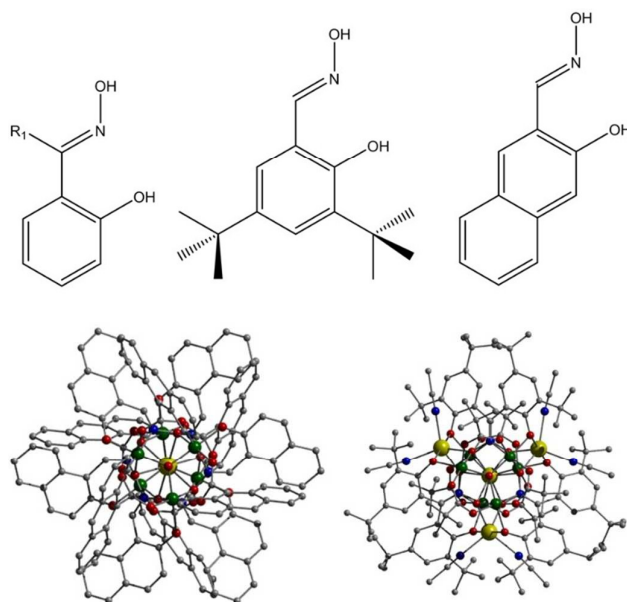
Figure 1 (Top) ChemDraw representations of the derivatised salicyaldoxime ligands used in this work (where R_1 = \text{Me, Ph} ). (Bottom) Crystal structure of 1 as viewed perpendicular (left) and parallel (right) to the \{\text{Cr(III)}_3\text{O}\}^{7+} planes. Colour code (used throughout this work): Cr (green), O (red), N (blue), Na (yellow), C (grey). All hydrogen atoms have been omitted for clarity.
