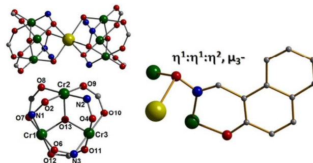
Figure 2 (Top left) Core in 1 highlighting the major connection pathways between the two \{\text{Cr(III)}_3\text{O}\}^{7+} triangular units and the central \text{Na}^+ ion. (Bottom left) Core in 1 illustrating the oximic (Cr-N-O-Cr) and carboxylate (Cr-O-C-O-Cr) bridges within the \{\text{Cr(III)}_3\text{O}\}^{7+} triangular units. (Right) Bonding mode exhibited by the Naphth-sao 2- ligands in 1 .
