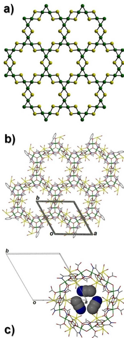
Figure 9 (a) Connectivity schematic taken from the crystal data of 5 illustrating its [3,6] net topology (colour code as used previously). (b) The [3,6] 2D extended network in 5 as viewed along the c axis of the unit cell. Solvent molecules of crystallisation (MeCN) have been omitted for clarity. (c) Three symmetry equivalent MeCN solvents of crystallisation (space-fill representations) lying perpendicular to the three fold axis along c and reside in-between the individual 2D sheets in 5 .
