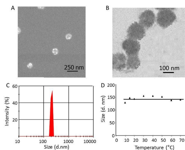
Fig. 1 p(\text{MVCA-co-SS}) : (A) SEM image; (B) TEM image; (C) size distribution diagram determined by DLS and (D) temperature dependence of the hydrodynamic diameter, DLS data (1 mg/ml, \text{H}_2\text{O} , 25 °C).
