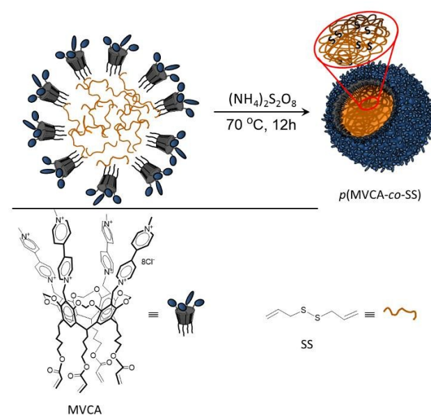
Scheme 1 Synthesis of p (MVCA-co-SS).
