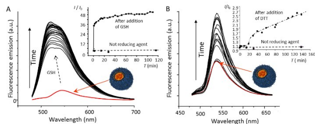
Fig. 4 Fluorescence spectra of FI@ p (MVCA-co-SS) (1 mg/ml) after addition of (A) GSH (0.3 mg/ml) and (B) DTT (1.2 mg/ml) (H 2 O, 25 °C). (inset) Intensity change at 550 nm in fluorescence spectra of FI@ p (MVCA-co-SS) after addition of the reducing agents.
