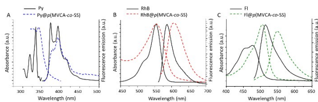
Fig. 3 UV-vis and fluorescence spectra of (A) Py, (B) RhB, (C) FI in aqueous media and encapsulated into p (MVCA-co-SS) (1 mg/ml, H 2 O, 25 °C).
