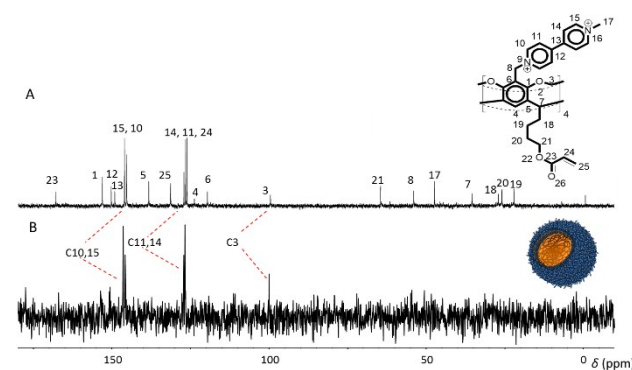
Fig. 2 ^{13}\text{C}\{^1\text{H}\} NMR spectra of (A) MVCA and (B) p(\text{MVCA-co-SS}) (600 MHz, \text{D}_2\text{O} ).
