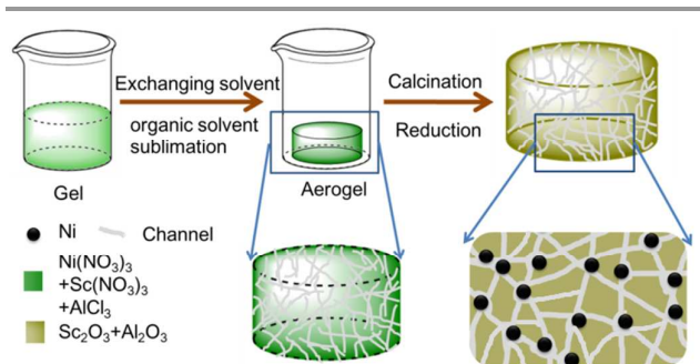
Scheme 1 Schematic diagram depicting the synthesis of NiSc/Al 2 O 3 -A catalysts.
