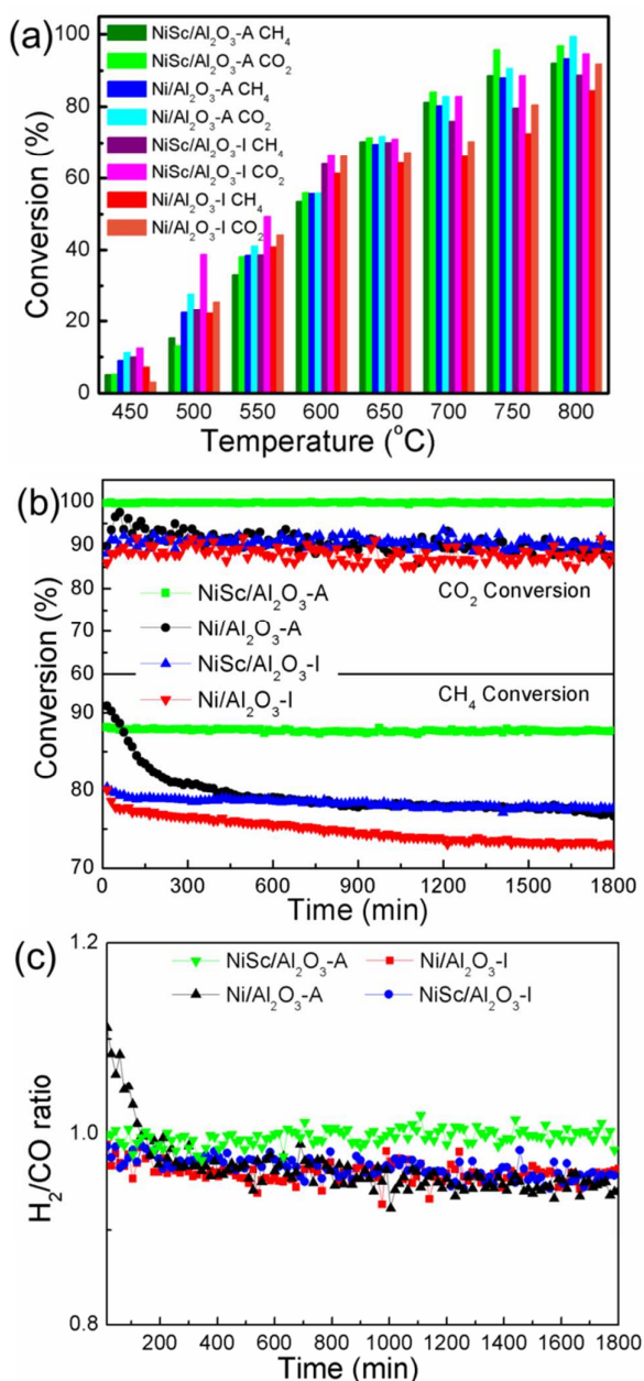
Fig. 6 (a) CH 4 and CO 2 conversions over various catalysts at different temperatures; (b) catalytic stability test and (c) H 2 /CO ratios of various catalysts for methane dry reforming at 750 °C for 1800 min. (Catalytic conditions: CH 4 :CO 2 = 1:1, 15 mL/min per reactor; 150 mg of catalysts.)
