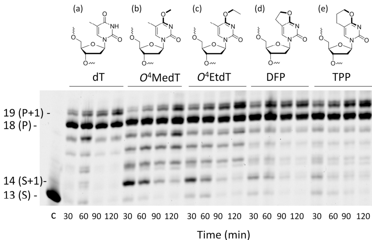
Figure 1: Structures of the (a) unmodified dT control, (b) O^4 MedT, (c) O^4 EtdT, (d) DFP and (e) TPP adducts. In bold are the bonds between the atoms shown to have a syn (b and c) or anti (d and e) orientation around the O^4 -C4 bond. Full primer extension assays for the control undamaged substrate (dT), O^4 MedT, O^4 EtdT, DFP, and TPP-bearing substrates with hPol \eta . The template strand sequence is 3'-AGCATTGCGAGTAXTACT-5' where X denotes the modification and the 5'-FAM labeled primer strand sequence is 5'-TCGTAAGCGUCAT-3'.
