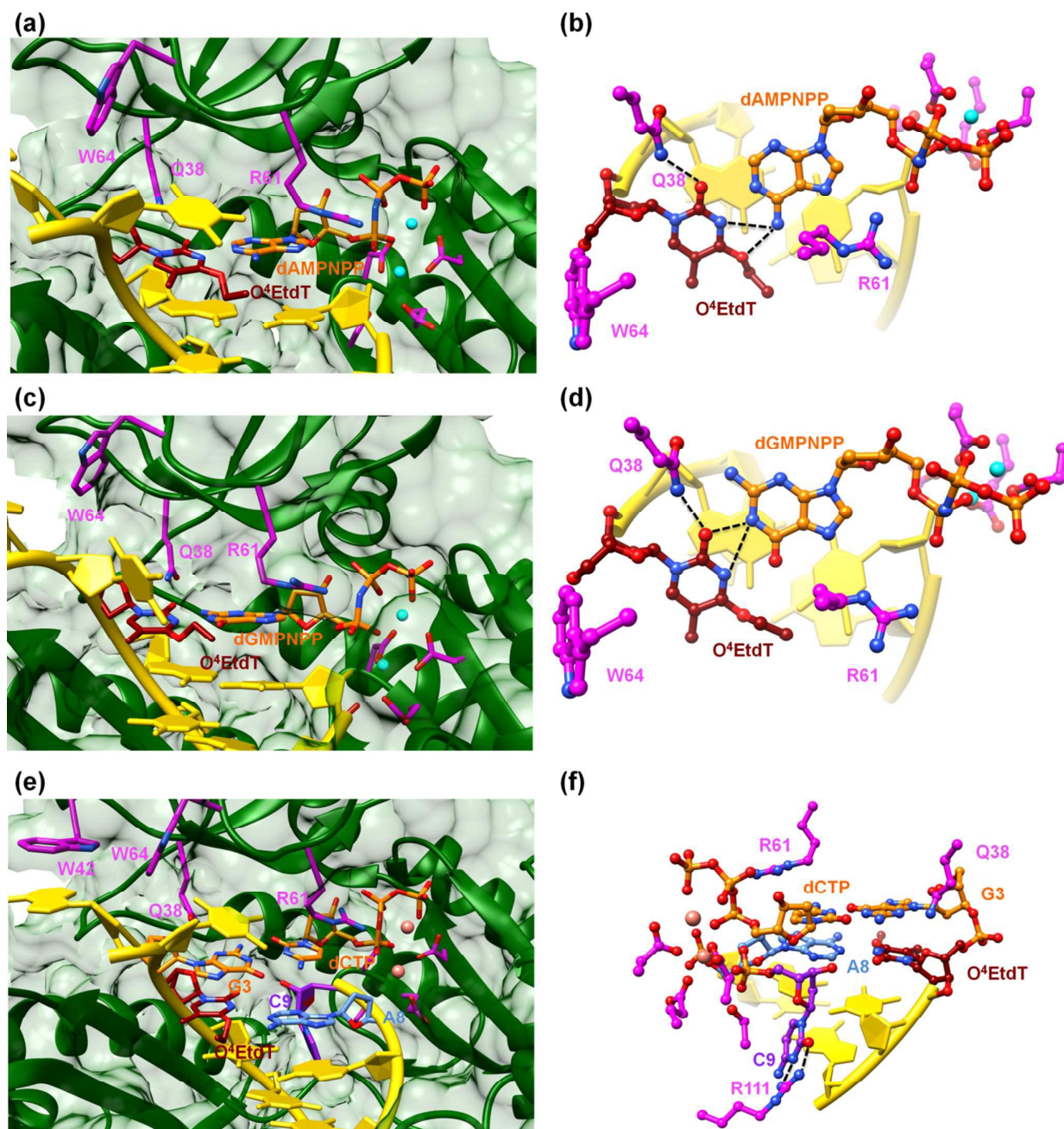
Figure 4: Pairing between incoming purine nucleotide triphosphate and O^4 EtdT in two hPol \eta insertion-stage complexes (a - d). (a), Major groove view of the Watson-Crick pair between dAMPNPP and O^4 EtdT with formation of bifurcated H-bonds. (b), The active site rotated by 90^\circ relative to A, with the base pair viewed perpendicular to the adenine plane. (c), Major groove view of the sheared configuration between dGMPNPP and O^4 EtdT, with formation of bifurcated H-bonds. (d), The active site rotated by 90^\circ relative to C, with the base pair viewed perpendicular to the guanine plane. Carbon atoms of O^4 EtdT, the incoming nucleotide triphosphate, and selected hPol \eta amino acid side chains are colored in maroon, orange and magenta, respectively. Mg^{2+} ions are cyan spheres and selected H-bonds are shown as dashed lines. Active site configuration in a ternary hPol \eta extension-step complex with O^4 EtdT opposite primer dA, followed by template dG opposite incoming dCTP (e - f). (e), Major groove view of the active site, with carbon atoms of O^4 EtdT and the paired dA colored in maroon and light blue, respectively. Carbon atoms of the nascent dG:dCTP pair are colored in orange, carbon atoms of selected hPol \eta amino acid side chains are colored in magenta, and those of the 3'-terminal primer dC are colored in purple. (f), The active site rotated by 180^\circ relative to A and viewed into the minor groove.
