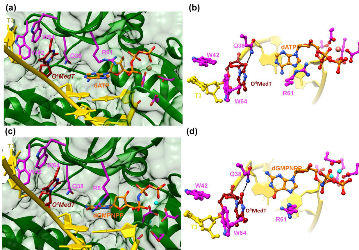
Figure 3: Detached arrangement of incoming purine nucleotide triphosphate and O^4 MedT in two hPol \eta insertion-stage complexes. (a), Active site conformation in the complex with dATP opposite O^4 MedT viewed into the DNA major groove, and (b), rotated by 90^\circ and viewed perpendicular to the adenine plane. (c), Active site conformation in the complex with dGMPNPP opposite O^4 MedT, viewed into the DNA major groove, and (d), rotated by 90^\circ and viewed perpendicular to the guanine plane. Carbon atoms of O^4 MedT, the incoming nucleotide triphosphate, and selected hPol \eta amino acid side chains are colored in maroon, orange and magenta, respectively. Mg^{2+} and Ca^{2+} ions are cyan and pink spheres, respectively, and selected H-bonds are shown as dashed lines.
