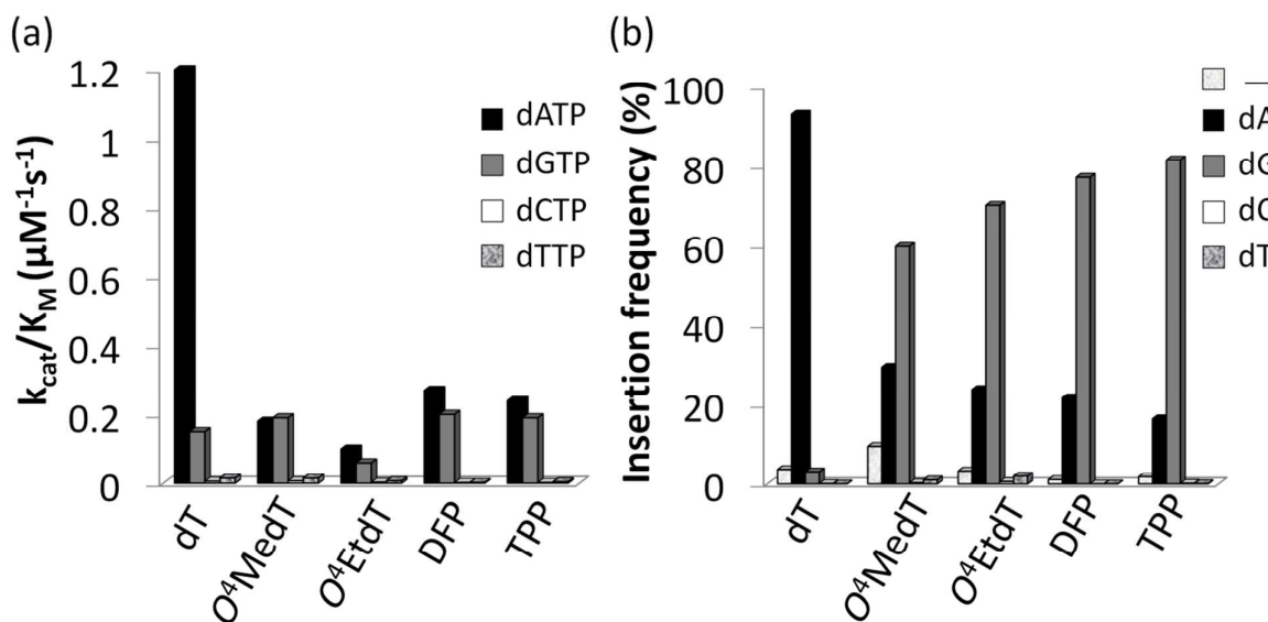
Figure 2: (a) Steady-state incorporation efficiencies opposite dT, O^4 MedT, O^4 EtdT, DFP, and TPP by hPol \eta with individual dNTPs. (b) Incorporation frequencies based on ESI-MS/MS analysis of primer extension products opposite the dT, O^4 MedT, O^4 EtdT, DFP, and TPP containing templates ("_" indicates frameshift adduct formation. Tabulated fragments identified by LC-MS/MS analysis of full-length extension products can be found in Supplementary Information).
