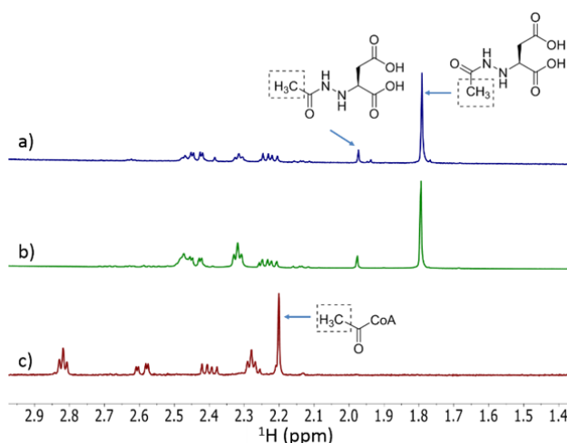
Fig. 3 1 H NMR spectra of the assay of His 6 -FzmQ with hydrazinosuccinate and Ac-CoA. a) 1 H NMR spectrum of the assay in panel b spiked with an authentic standard of N -acetylhydrazinosuccinate. b) NMR spectrum of the reaction mixture containing hydrazinosuccinate, Ac-CoA, and His 6 -FzmQ. c) NMR spectrum of the reaction mixture in the absence of His 6 -FzmQ. Note: Both enzymatically prepared and synthetic N -acetylhydrazinosuccinate exist as a pair of rotational isomers (see ESI†).
