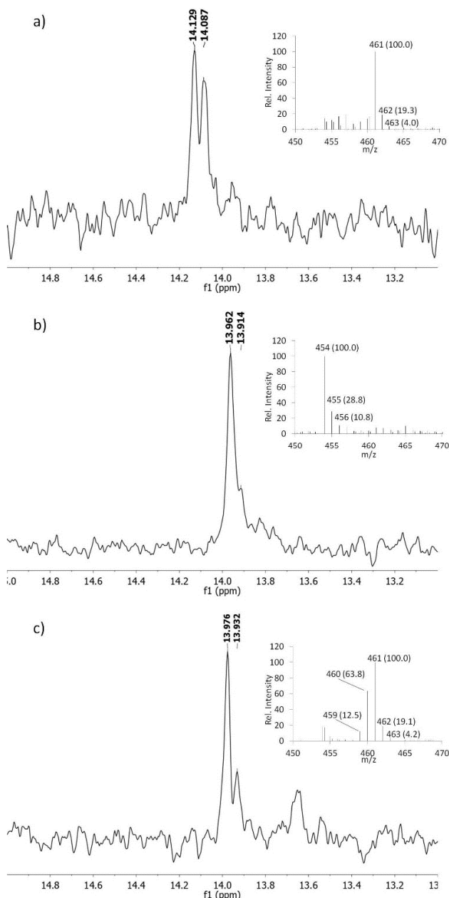
Fig. 5 31 P NMR spectra of fosfazinomycin produced by Streptomyces sp. NRRL S-149. The strain was grown on 15 NH 4 Cl and 15 N-Asp (top), NH 4 Cl and 15 N-Asp (middle), and 15 NH 4 Cl and unlabelled Asp (bottom). MS data for each spectrum are shown as insets. 31 P NMR chemical shifts for phosphonates are sensitive to pH because their pK a,2 is close to the pH of the producing medium. Hence, the three samples show slightly different chemical shift values.
