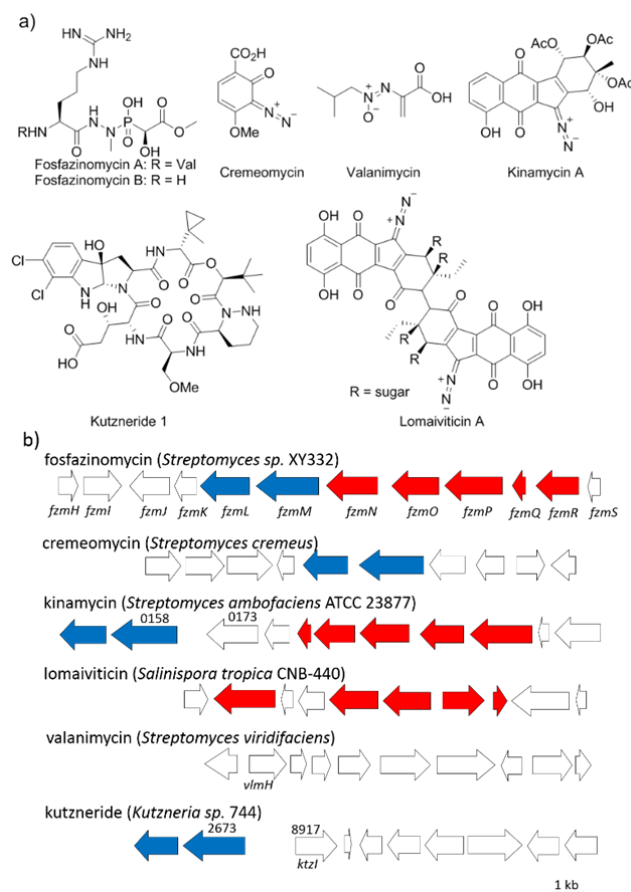
Fig. 1 a) Structures of a selection of compounds containing N-N bonds for which the biosynthetic gene clusters have been reported. b) Partial biosynthetic gene clusters of the compounds shown in panel a. Genes conserved in fosfazinomycin and lomaiviticin clusters are shown in red, whereas genes conserved in fosfazinomycin and cremeomycin clusters are shown in blue. The locus numbers of the genes are labelled above the genes.
