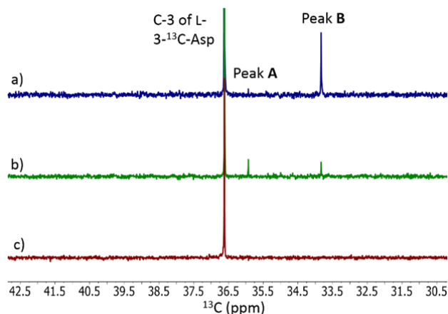
Fig. 4 13 C NMR analysis of the activity of His 6 -FzmM on L-3- 13 C-Asp. a) Same as panel b except the spectrum was recorded after incubation for 5 h. b) NMR spectrum of the reaction mixture containing L-3- 13 C-Asp, FAD, NADPH, O 2 , and His 6 -FzmM after incubation for 10 min. c) NMR spectrum of the reaction mixture in the absence of His 6 -FzmM after incubation for 23 h.
