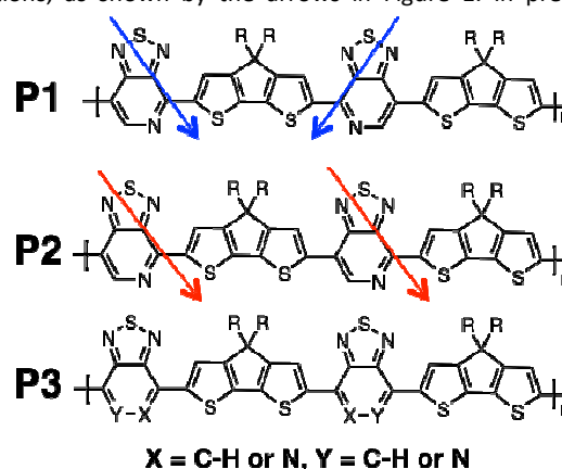
Figure 1. Polymers of interest in this study. experimental work, it was found that the hole mobilities between the regioregular arrangement of these CDT and PT units differ by orders of magnitude, with the regioregular polymers having higher hole mobilities. 13
