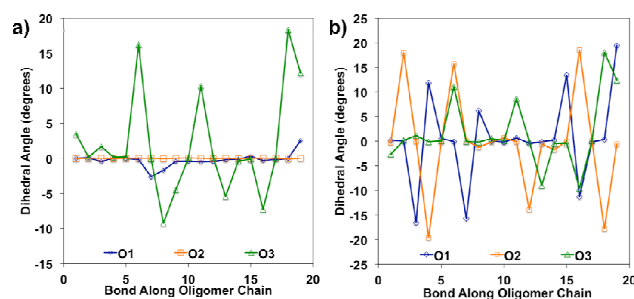
Figure 5. Dihedral angles along the oligomer backbone for (a) neutral oligomers and (b) relaxed cation oligomers, calculated in solvent environment.
