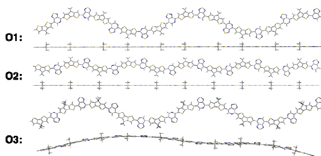
Figure 2. Optimized geometries of O1-O3 in solvent environment.
