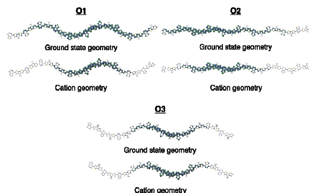
Figure 3. Cation spin density of O1-O3 in the ground state optimized geometry and the cation optimized geometry.
