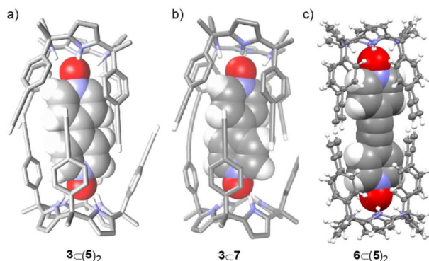
Fig. 2 a) PM6 energy minimized structure of the 3 ⊂( 5 ) 2 homocapsule. b) PM6 energy minimized structure of the putative complex formed by dimeric species 7 and guest 3 . For clarity, some non-polar hydrogen atoms from the host are removed. Guest molecules are shown as CPK models and calix[4]pyrrole 5 is depicted in stick representation. c) X-ray structure of the 6 ⊂( 5 ) 2 homocapsule shown in ORTEP representation with thermal ellipsoids set at 50% probability and hydrogen atoms as fixed spheres of 0.3 Å radius.
