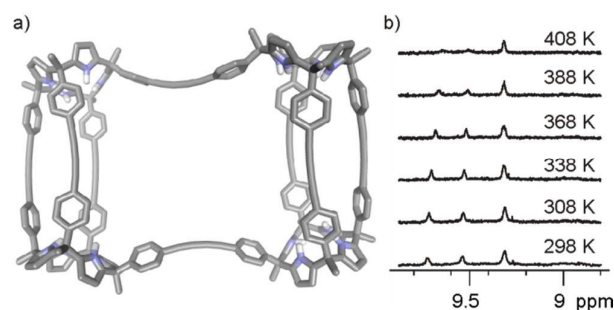
Fig. 6 a) MM3 energy minimized structure of a putative transition state structure for the racemization process of (M,P) -( 6 ) 2 ⊂ 9 . Guest molecules and hydrogens atoms were omitted for clarity. b) Selected 1 H NMR regions (NH pyrrole protons) of the variable temperature experiments performed using a solution of ( 6 ) 2 ⊂ 9 in Cl 2 CDCl 2 .
