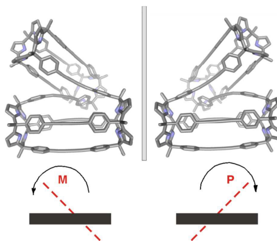
Fig. 5 X-ray crystal structures of the enantiomeric conformers of the (6)_2\subset 9 tetramer present in the crystal lattice. The M and P nomenclature was used to assign the absolute configuration of the two helimers. Hydrogen atoms and the encapsulated guest molecules were omitted for clarity.
