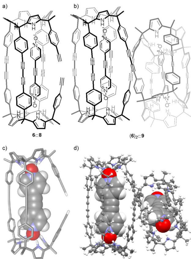
Fig. 4 Line-drawing structures of compounds: a) 6\subset 8 and b) (6)_2\subset 9 ; c) PM6 energy minimized structure of 6\subset 8 and d) X-ray crystal structure of (6)_2\subset 9 shown in ORTEP representation with thermal ellipsoids set at 50% probability and hydrogen atoms as fixed spheres of 0.3 Å radius.
