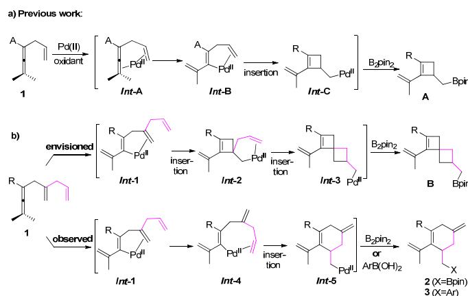
Scheme 1. Previous reports and this approach.
