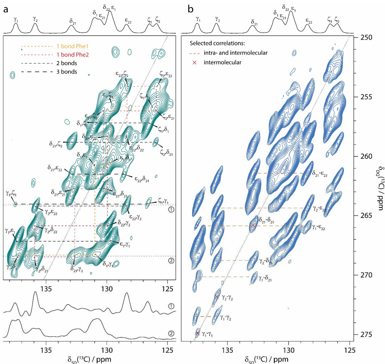
Fig. 4. Aromatic region of ^{13}\text{C} - ^{13}\text{C} DQ-SQ correlation spectra of cyclo-FF, obtained with the dipolar recoupling sequence S_3 applied during total recoupling times (DQ excitation plus reconversion) of 2.3 ms (a) and 13.8 ms (b). The spectra were recorded in \sim 18.5 h (a) and \sim 7.4 h (b), respectively. ^{13}\text{C} CPMAS spectra are shown above for illustrative purposes. Note the overlapping \delta_1 and \epsilon_1 resonances of one of the phenyl rings compared to resolved resonances ( \delta_{21} , \delta_{22} , \epsilon_{21} and \epsilon_{22} ) for the second ring. The up- and downfield shifts of \epsilon_{22} and \delta_{21} , respectively, are signs of intermolecular interactions, in this case of parallel \pi -stacking. 5,15 Cross sections along the black dotted lines ( \delta_{DQ} = 264.1 ppm and \delta_{DQ} = 268.5 ppm) in (a) are displayed below and show the narrowing of linewidths for long distance peaks (upper cross section, linewidths 40–50 Hz) compared to cross-peaks arising from directly bonded carbons (lower cross section, linewidths >100 Hz). Resolved cross-peaks used for the buildup analysis (see Fig. 5) are labeled in (b). Among them, select pure intermolecular peaks are marked by a red cross, and select peaks resulting from intra- and intermolecular contributions are connected with an orange dashed line.
