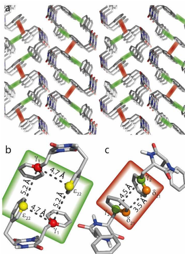
Fig. 6 (a) Crystal structure of cyclo-FF 15 with perpendicular and parallel \pi - \pi interactions highlighted in green and red, respectively. (b-c) Close-up of perpendicular (b) and parallel (c) \pi -stacking. The highlighted distances can be probed by the 2D experiments presented in this paper. Note that the relevant carbon atoms and distances are highlighted for illustrational purposes on the same pair of cyclo-FF molecules. However in a sample at NA, it is highly unlikely to have four 13 C isotopes occurring in only two cyclo-FF molecules. The highlighted distances contribute individually to the polarization transfer in different molecule pairs across the sample.
