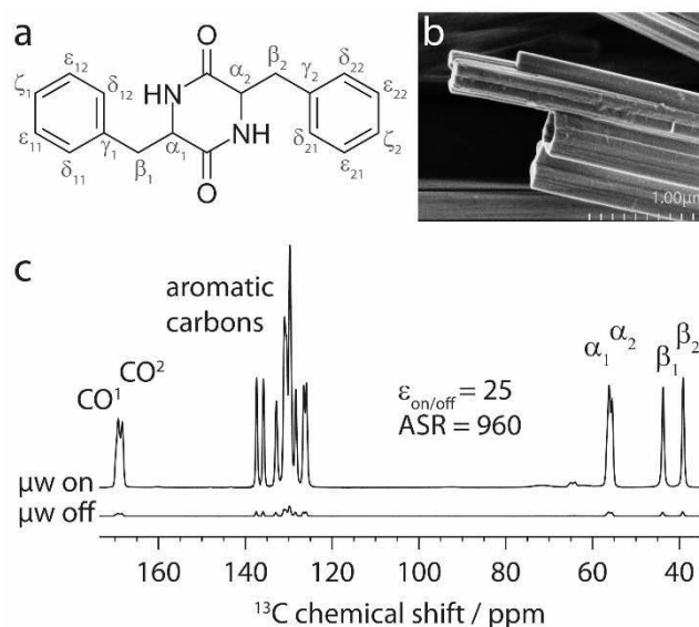
Fig. 1 (a) Chemical structure of cyclo-FF. (b) Scanning electron microscopy image of cyclo-FF nanotubes. (c) 13 C CPMAS spectra of cyclo-FF with and without microwave ( \mu\text{w} ) irradiation. \epsilon_{\text{on/off}} describes the ratio of peak heights of the two spectra. The ASR is the ratio of the signal-to-noise per unit square root of time between the spectrum recorded with \mu\text{w} irradiation and a CPMAS spectrum taken in a conventional ssNMR experiment.
