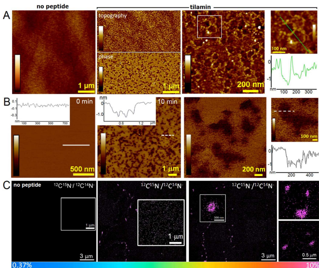
Fig. 4. Monolayer poration in reconstituted membranes. Topographic (AFM) and chemical (NanoSIMS) imaging of DLPC/DLPG (3:1, molar ratio) SLBs. (A) In-air AFM topographic images with a cross-section along the highlighted line (green) shown for the inset. Colour scales: 3 nm for the topography images; and 15 degrees for the phase image. Incubation conditions: 10 μM, pH 7.4, rt. (B) Topography of supported lipid bilayers measured by AFM in aqueous solution during incubation with tilamin where 0 min corresponds to the time of tilamin injection. Colour scale: 3 nm. Incubation conditions: 1.8 μM, pH 7.4, rt. (C) SIMS images of ^{12}\text{C}^{15}\text{N}^-/^{12}\text{C}^{14}\text{N}^- ratio obtained for the tilamin-treated DLPC/DLPG (3:1, molar ratio) SLBs, and expressed as hue saturation images, which are the sums of sequential images to enhance the statistical significance of the measured ratios. The rainbow scale changes from blue (natural abundance of 0.37%) to pink (10%). Insets for tilamin-treated bilayers highlight pore clusters (middle and right), and no clusters in untreated bilayers (left). Incubation conditions: 10 μM, pH 7.4, rt.
