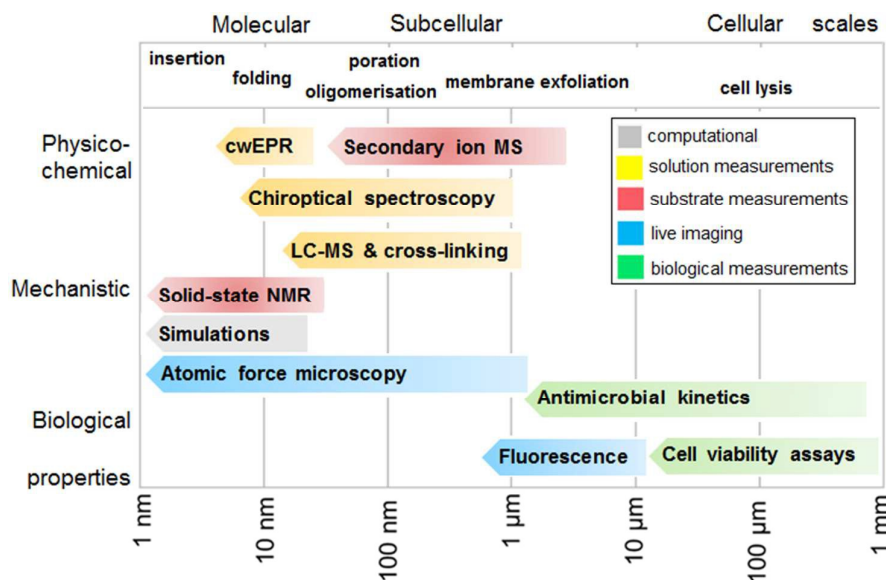
Fig 2. Measurement continuum. A schematic representation of a molecular-to-cellular scale measurement continuum used to demonstrate antimicrobial monolayer poration. Key: cwEPR: continuous wave electron paramagnetic resonance, MS: mass spectrometry, LC-MS: liquid-chromatography mass spectrometry, NMR: nuclear magnetic resonance spectroscopy.
