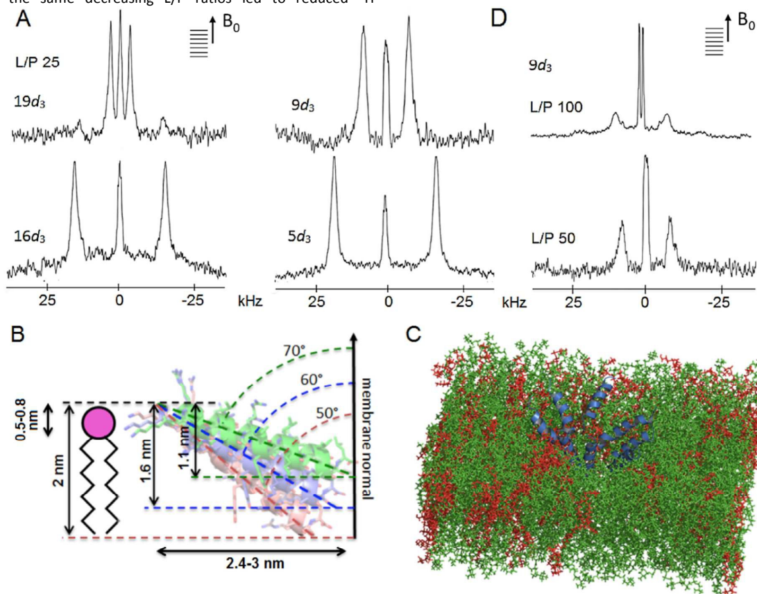
Fig. 6. Tilamin insertion mode. (A) Oriented ^2\text{H} NMR quadrupolar splittings ( \Delta\nu\text{Q} ) in palmitoyl (POPC/POPG, 3:1 molar ratio) membranes for tilamin deuterated (Ala- d_3 ) at positions 19, 16, 9, 5 at a lipid-peptide (L/P) ratio 25. (B) A GALA-derived and MD-derived ensemble of helix tilt angles for tilamin in the outer leaflet of the phospholipid bilayer showing tilt angles with corresponding insertion depths and horizontal spans of the tilted helix. The helices are not to scale. The helix insertion by the C-terminus (Solution 2) is shown (Table S4). (C) A rudimentary low-oligomer pore constructed by coarse-grained molecular dynamics simulations and converted to atomistic coordinates in a newly equilibrated palmitoyl (POPC/POPG, 3:1 molar ratio) membrane. Membrane slabs are oriented to view the peptide tilts. Peptides, POPC and POPG lipids are in blue, green and red, respectively. (D) Oriented ^2\text{H} NMR quadrupolar splittings ( \Delta\nu\text{Q} ) in palmitoyl (POPC/POPG, 3:1 molar ratio) membranes for tilamin deuterated (Ala- d_3 ) at position 9 at L/P ratios 100 and 50.
