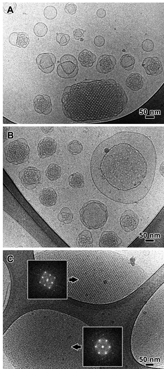
Figure 4. Cryo-TEM images of self-assembled MO/P80 and MO/P80/ \beta -CD- n C 10 nanocarriers obtained upon amphiphile dispersion in the presence of 5 mol% P80 surfactant stabilizer with respect to the nonlamellar lipid MO. (A,B) MO/5 mol% P80 assemblies; (C) MO/5 mol% P80/4 mol% \beta CD- n C 10 assemblies. Insets: FFT spectra of the regions indicated by arrows. Aqueous phase: Milli-Q water.
