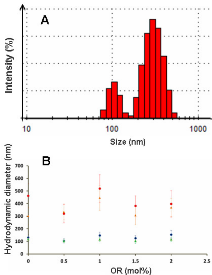
Figure 6. (A) Quasi-elastic light scattering (QELS) results showing a bimodal distribution of hydrodynamic particle diameters in MO/P80/ \beta CD-nC 10 dispersed systems loaded with Oil red (OR). (B) Dependence of the hydrodynamic diameters on the molar content of OR. The OR content in the mixed amphiphilic films used for nanocarrier preparation is 0.5, 1, 1.5 and 2 mol% with respect to MO. The triangles indicate the MO/P80/ \beta CD-nC 10 systems, whereas the circles correspond to MO/P80 systems lacking \beta -CD-nC 10 . The two populations of nanoparticles may be attributed to small cubosomal intermediates and vesicular membranes ( D_h \sim 80 -120 nm) (blue and green symbols), which coexist with well developed liquid crystalline cubic lattice assemblies (cubosomes) of D_h \sim 250 -500 nm (red symbols). Aqueous phase: MilliQ water.
