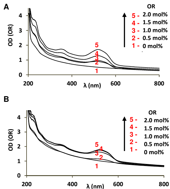
Figure 7. Optical density (OD) plots derived from recording of UV-Vis spectra of Oil red (OR) solubilized in aqueous dispersions of MO/P80 and MO/P80/ \beta CD- n C 10 nanocarriers. The dispersed systems are prepared from mixed films containing 0.5, 1.0, 1.5 and 2 mol% OR with respect to the nonlamellar lipid MO. Temperature is 25 °C. Aqueous phase: Milli-Q water.
