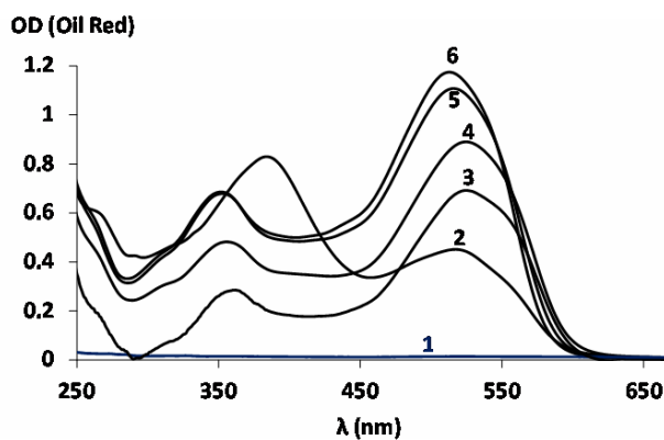
Figure 8. Comparison of the UV-Vis spectra of Oil red (OR) solubilized in organic solvents of variable polarities (1: water, 2: chloroform; 4: ethylene glycol, 5: ethanol, 6: acetonitrile) with that of OR in amphiphilic nanoassemblies constituted of monoolein (MO), polysorbate 80 (P80) and \beta -CD- n C 10 (3: MO/P80/ \beta -CD- n C 10 ) after subtraction of the nano-objects scattering. The concentration of Oil red in the organic solutions is 0.04 mM. Temperature is 25 °C.
