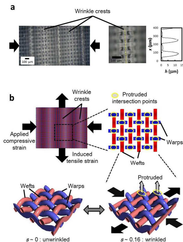
Fig. 3. Fine structures on wrinkled surface. (a) An optical image of wrinkle crests at s = 0.16 with the cross-sectional profile measured separately along the crest, indicated by the yellow broken line in the middle image. (b) Schematic explanation for the induced local protrusions of warps at the intersection points on the wrinkled surface. The yellow circles indicate the intersection points where warps lay over wefts. In the three-dimensional illustrations, only the local structural change in the textile sheet is shown. The large undulation of wrinkles and the PDMS of layer-A, which embeds the textile sheet, is not shown for the sake of simplicity.
