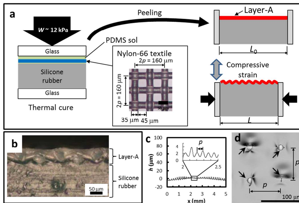
Fig. 1. Textile-embedded elastomer sample. (a) Schematic illustration for sample fabrication. (b) Cross-sectional image and (c) surface profile of sample surface at s = 0 . (d) Optical image of sample surface at s = 0 . Note that the skin of the PDMS on the intersection point is partially peeled by a diameter of 15–25 \mu\text{m} , indicated by arrows.
