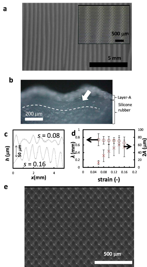
Fig. 2. Surface of textile-embedded elastomer under uniaxial compressive strain. (a) Optical image at s = 0.16 applied in horizontal direction. (b) Cross-sectional image of the sample shown in (a). The undulation in the soft foundation is confirmed from the undulating streaks indicated by the white arrow with the dashed line for guides for eyes. (c) Representative cross-sectional profiles of sample surfaces along the strain direction. (d) Plots of wavelength \lambda (circles) and amplitude 2A (crosses) with respect to applied strain s . (e) Optical image at s = 0.16 in the bias direction, which is the horizontal direction in the image, showing no wrinkle.
