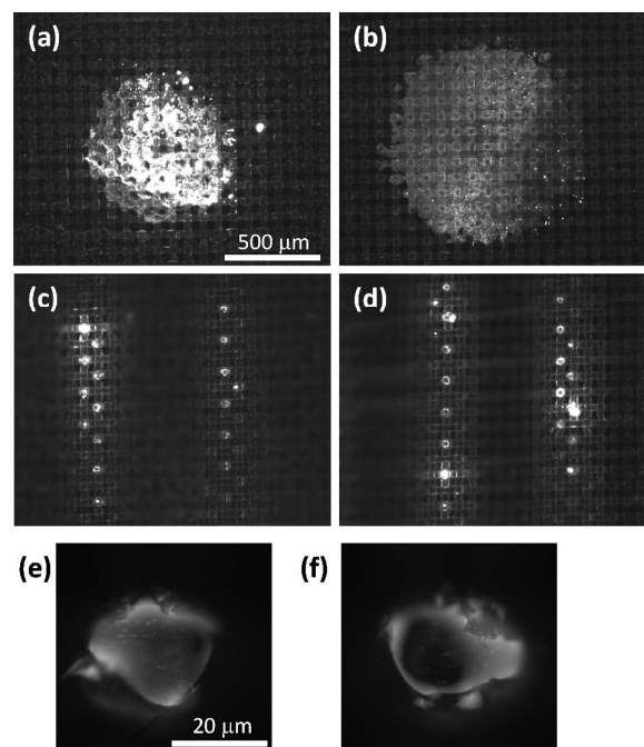
Fig. 6. Typical fluorescent images for estimation of contact state during friction on uncrinkled ( s = 0 ) and wrinkled ( s = 0.16 ) surfaces. The indenter coated with fluorescent ink was stamped at (a) s = 0 , P = 29.4 mN, (b) s = 0 , P = 196.0 mN, (c) s = 0.16 , P = 29.4 mN, and (d) s = 0.16 , P = 196.0 mN. (e) and (f) Representative magnified images of the apparent contact points on wrinkled state. Although the edge of the fluorescent part appears brighter, the inner part also shows fluorescence, suggesting the contact of the top of the nylon-66 fibre with the indenter.
