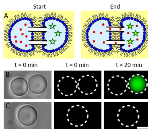
Fig. 4 Confirmation of DIB assembly by showing the interdroplet exchange of calcium ions (A) Schematic drawing illustrating the movement of calcium ions (red dots) through \alpha\text{HL} nanopores inserted into the DIB into the neighbouring droplet containing the calcium sensitive dye Fluo-4 (stars). (B) Droplets containing Fluo-4, \alpha\text{HL} and EDTA in buffer were manipulated into contact with droplets containing calcium chloride and \alpha\text{HL} in buffer (circles). (C) A single droplet containing Fluo-4, \alpha\text{HL} and EDTA in buffer was used as a control (squares). Scale bar = 10 \mu\text{m} .
