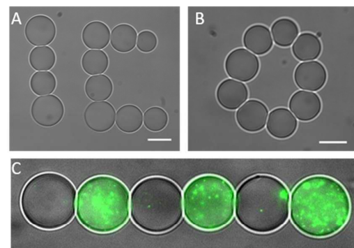
Fig. 2 The assembly of symmetric and asymmetric 2D OptiDIB networks using optical tweezers. (A) A linear and a branched 2D network (scale bar = 15 \mu\text{m} ) and (B) a circular 2D network (scale bar = 10 \mu\text{m} ) assembled from one droplet type. (C) A linear asymmetric OptiDIB network formed from alternating droplet types (scale bar = 15 \mu\text{m} ). (D) An asymmetric 2D OptiDIB ‘X’ network consisting of alternating droplet types (scale bar = 15 \mu\text{m} ). Images in panel C and D were obtained by superimposing the brightfield and fluorescence micrographs. (E) A complex 2D OptiDIB network assembled from three droplet types. The position and identity of the droplets is highlighted by the dashed outlines (scale bar = 15 \mu\text{m} ).
