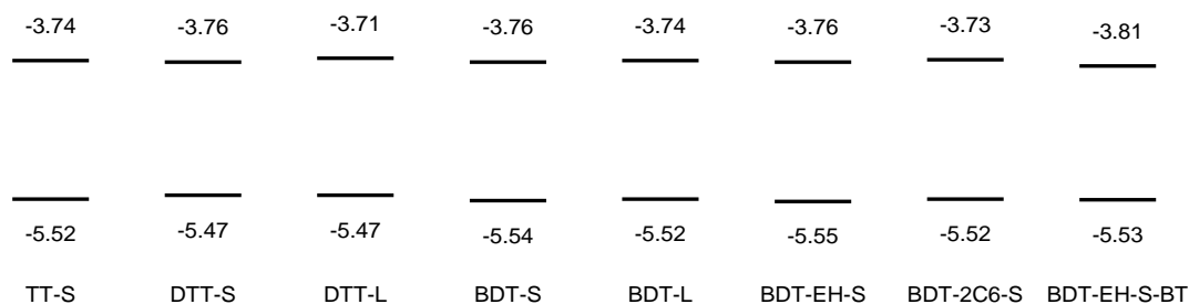
Fig. 3 Energy levels (in eV vs. vacuum) of bis-DPP molecules measured by cyclic voltammetry.
