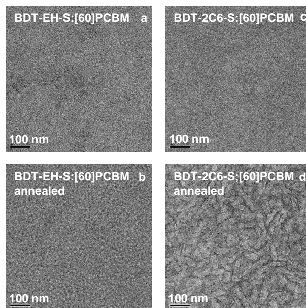
Fig. 5 TEM images of optimized photoactive layers of BDT-EH-S (a,b) and BDT-2C6-S (c,d) spin coated from chloroform containing 0.2% 1-CN before (a,c) and after (b,d) thermal annealing at 110 °C for 10 min.
