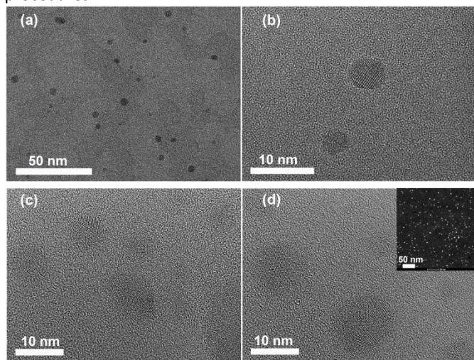
Figure 2. High-resolution TEM (HRTEM) images of Au (a, b) and Ag NPs (c, d); the inset: STEM) generated by the HFS at 1 kHz, showing their shape and configuration and confirming their crystal structure.
