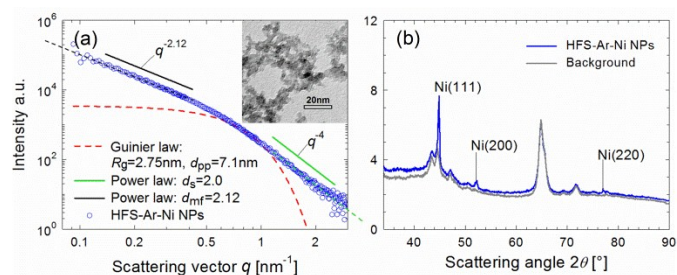
Figure 4. SAXS/WAXS and TEM measurements of Ni NPs generated at 3 kHz. (a) SAXS curve and TEM image (inset), which provides the small primary particles of a few nm in size. (b) WAXS curves
