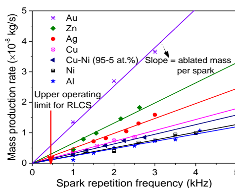
Figure 1. Mass production rates of HFS-produced Au, Zn, Ag, Cu, Cu-Ni (95-5 at.%), Ni, and Al NPs, as a function of spark repetition frequencies. Symbols denote the gravimetric measurements of the electrodes, while the lines are fits to the measurements. The red arrow indicates the upper operating limit of the RLCS.
