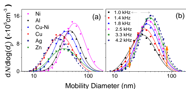
Figure 3. Size distributions of agglomerated NPs produced by the HFS for (a) Ni, Al, Cu-Ni (95-5 at.%), Cu, Ag, and Zn NPs produced at 1 kHz, and (b) Cu NPs produced using different spark repetition frequencies. The symbols denote the SMPS measurements and the curves are fitted log-normal distributions to the data.
