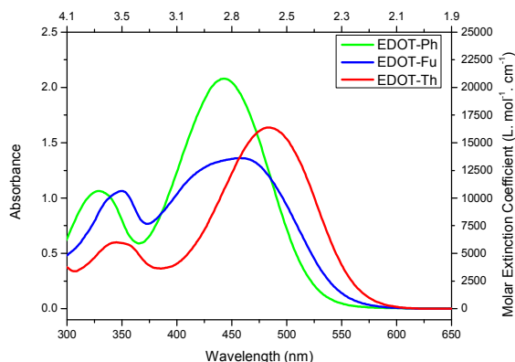
Fig. 1 UV-vis absorbance spectra of dyes EDOT-Ph , EDOT-Fu and EDOT-Th (THF 1 \times 10^{-4} M).
