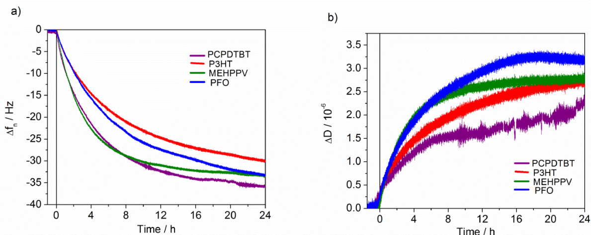
Figure 5. Representative normalized frequency (a) and dissipation (b) shifts upon fibronectin adsorption for the polymers surface (overtone n = 9 )
