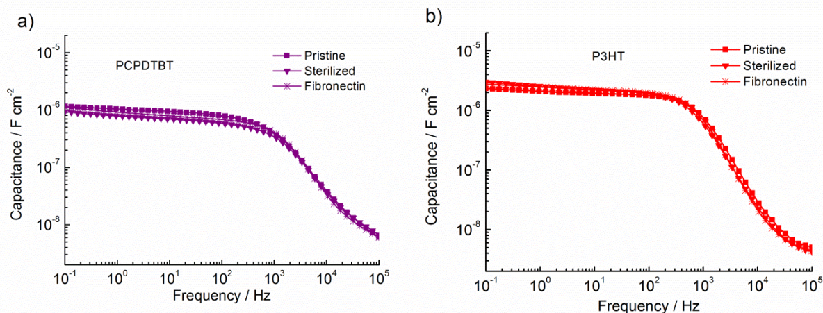
Figure 8. Capacitance values versus frequency extrapolated from the corresponding equivalent circuit derived from impedance measurements for pristine polymers, sterilized polymers and polymers after protein incubation. a) PCPDTBT; b) rr-P3HT
