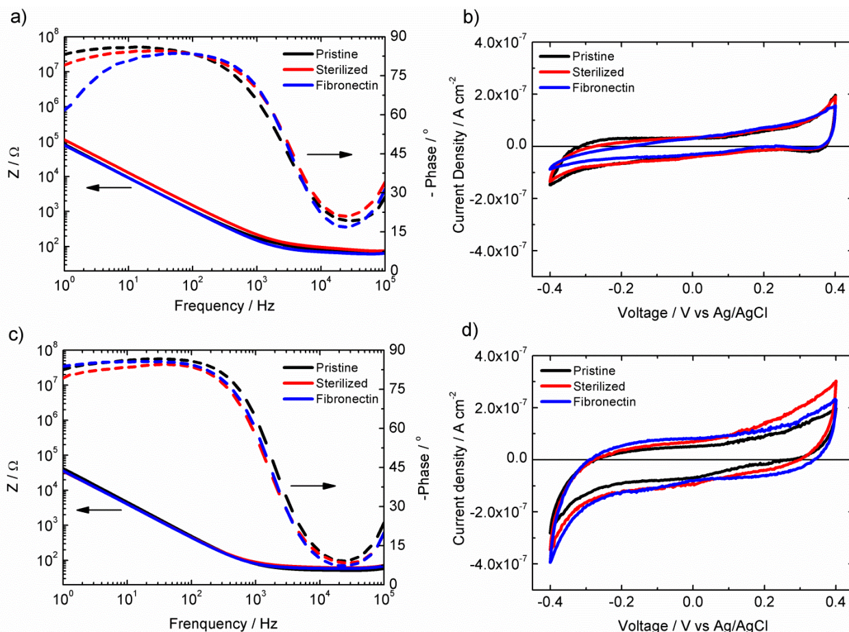
Figure 7. Electrochemical measurements of PCPDTBT (top) and rr-P3HT (bottom), as deposited (black line), after sterilization (red line), and after protein incubation (blue line), in 0.2 M NaCl. a) and c) Bode plot for PCPDTBT and rr-P3HT, respectively.
