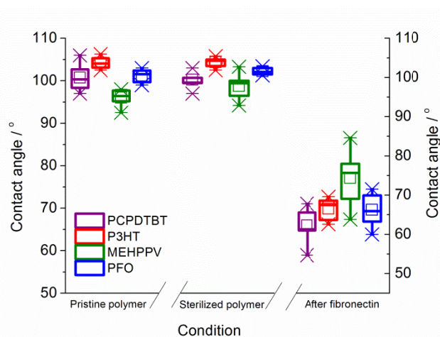
Figure 1. Static water contact angles for the different polymers investigated.
