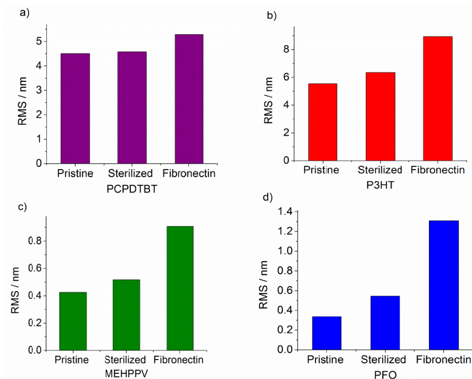
Figure 4. RMS measured at 1 \mu\text{m} length scales. a) PCPDTBT, b) rr-P3HT, c) MEH-PPV and d) PFO
