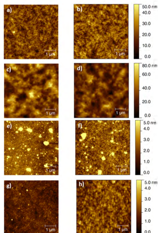
Figure 2. AFM topography images of pristine (left) and sterilized polymers (right) (sample area, 5 \times 5 \mu\text{m}^2 ). From top to the bottom: PCPDTBT, rr-P3HT, MEH-PPV and PFO.
