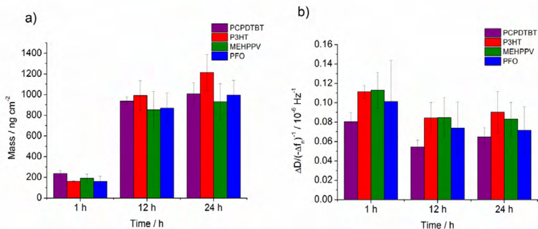
Figure 6. a) QCM-D modelling results for the mass of fibronectin adsorbed on the different polymers at 1 h, 12 h and 24 h. b) \Delta D/(-\Delta f_n)^{-1} data for fibronectin adsorption onto the different polymers at 1 h, 12 h and 24 h (overtone n = 9 ). Data are reported as average values \pm SD ( n = 3 samples for each polymer type). No statistically significant difference was observed among the different polymers (Student's t -test, P value > 0.1 in all cases).
