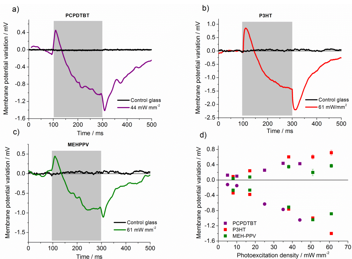
Figure 10. a-c) Representative membrane potential variation measured in HEK-293 cells ( n = 10 per each type of polymer) cultured on different photoactive polymers under illumination (grey area in the plot indicates light on). PCPDTBT excitation wavelength peak, \lambda = 635 nm; P3HT and MEH-PPV, \lambda = 475 nm. Black lines refer to control samples, with cells cultured on top of glass substrates and under the same photoexcitation density used for the corresponding polymer (d) Variation of depolarization and hyperpolarization signals of conjugated polymers with increasing photoexcitation density. PCPDTBT (violet symbols) was excited at \lambda = 635 nm, in a range between 5 and 44 mW mm -2 ; rr-P3HT (red symbols) and MEH-PPV (green symbols) were excited at \lambda = 475 nm, in a range between 8 and 61 mW mm -2 . Depolarization data correspond to the maximum depolarization peak; hyperpolarization data were obtained as the average value over the last 15-ms illumination period.
