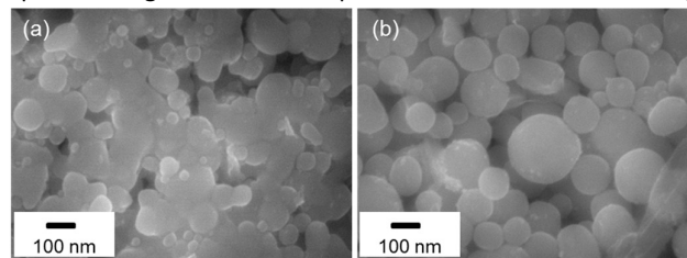
Figure 5. SEM images of the surface of Sn patterns made of Sn NPs synthesized using: (a) 0.0089 g PVP (Sn NPs of 37.8 \pm 12.5 nm), (b) 0.0018 g PVP (Sn NPs of 88.6 \pm 21.3 nm).
