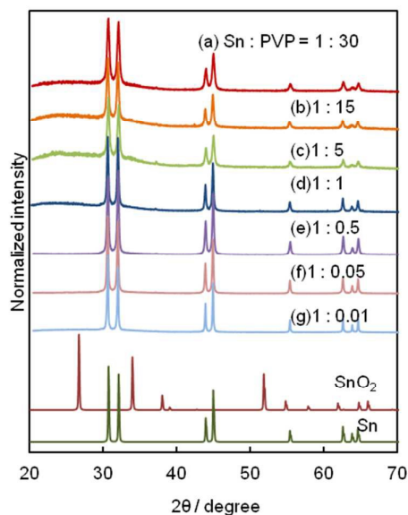
Figure 1. XRD patterns of Sn NPs synthesized using different amounts of PVP: (a) 5.3420, (b) 2.6710, (c) 0.8903, (d) 0.1781, (e) 0.0890, (f) 0.0089, and (g) 0.0018 g. The corresponding weight ratios of the input elemental Sn to PVP were indicated inset. The reference patterns of tetragonal \text{SnO}_2 (JCPDS no. 41-1445) and Sn (JCPDS no. 04-0673) are also shown.
