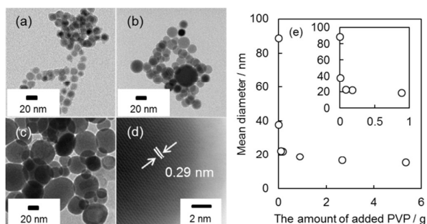
Figure 2. TEM images of Sn NPs synthesized using different amounts of PVP: (a) 5.3420, (b) 0.0890, and (c) 0.0089 g; (d) HRTEM image of a Sn NP (25 nm) obtained using PVP of 0.0890g; (e) average diameter of Sn NPs synthesized with various amounts of PVP from 0.0018 to 5.3420 g. The inset shows the expansion plots of (e) from 0 to 1.0 g of the input PVP.
