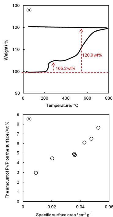
Figure 3. (a) A TGA curve of Sn NPs synthesized using 0.1781 g of PVP, (b) the relation between the specific surface area of Sn NPs and PVP amount on the NP surface.
