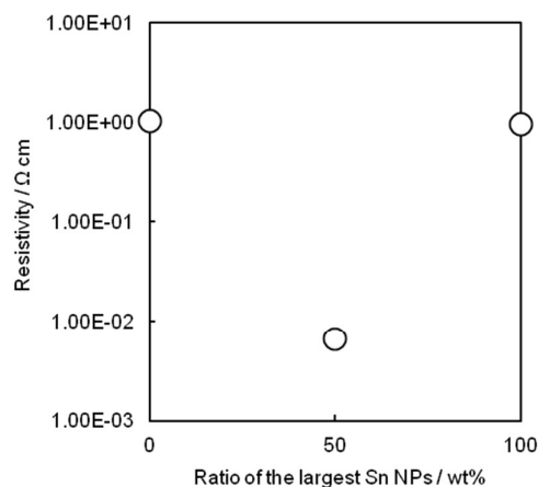
Figure 6. Resistivity of Sn patterns prepared from the smallest Sn NPs ( 15.2 \pm 3.1 nm), the largest Sn NPs ( 88.6 \pm 21.3 nm), and their mixture at 50 wt%.
