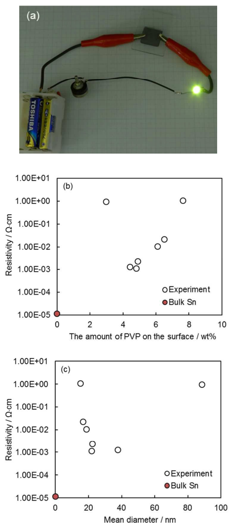
Figure 4. (a) An optical photograph of the conductive Sn pattern allowing electrical connection to light-up a LED tip. The resistivity of the Sn conductive patterns as a function of (b) the PVP amount on the surface of Sn NPs and (c) the NP size. A red point is for the resistivity of the bulk Sn.
