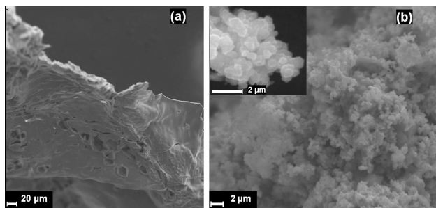
Fig. 3 SEM images illustrating the contrast in microstructure for (a) 1 and (b) 3 .
