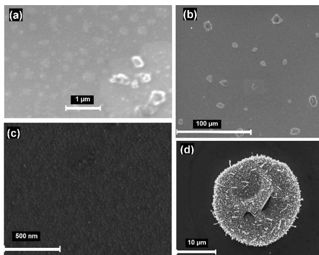
Fig. 5 SEM images of films: (a) as initially deposited on the Si substrate by spin coating (sample D); (b) after deposition by spin coating and subsequent heating under ammonia (sample L); (c) showing a continuous layer in sample L after ammonolysis; (d) showing a single "island" formed after ammonolysis at higher magnification (sample E).
