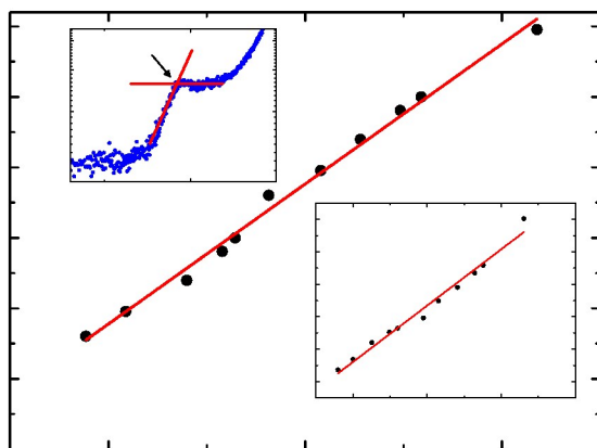
Fig. 5 Critical scaling behaviour of TEA(TCNQ) 2 analogous to spin glass systems where the critical temperature varies with frequency. Top inset: A graph showing how the transition temperature ( T_{ST} ) was defined. Bottom inset: Mydosh-type analysis of through the transition to study the frequency dependence and to get a value for T_0 within this magnetic transition. In all cases errors are given in brackets.
