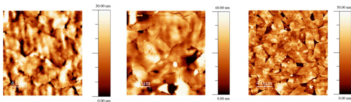
Figure 5: AFM images of OFETs fabricated from 5T-TTF (left), 5T-TTF + 5% CZTS (centre) and 5T-TTF + 10% CZTS (right)
