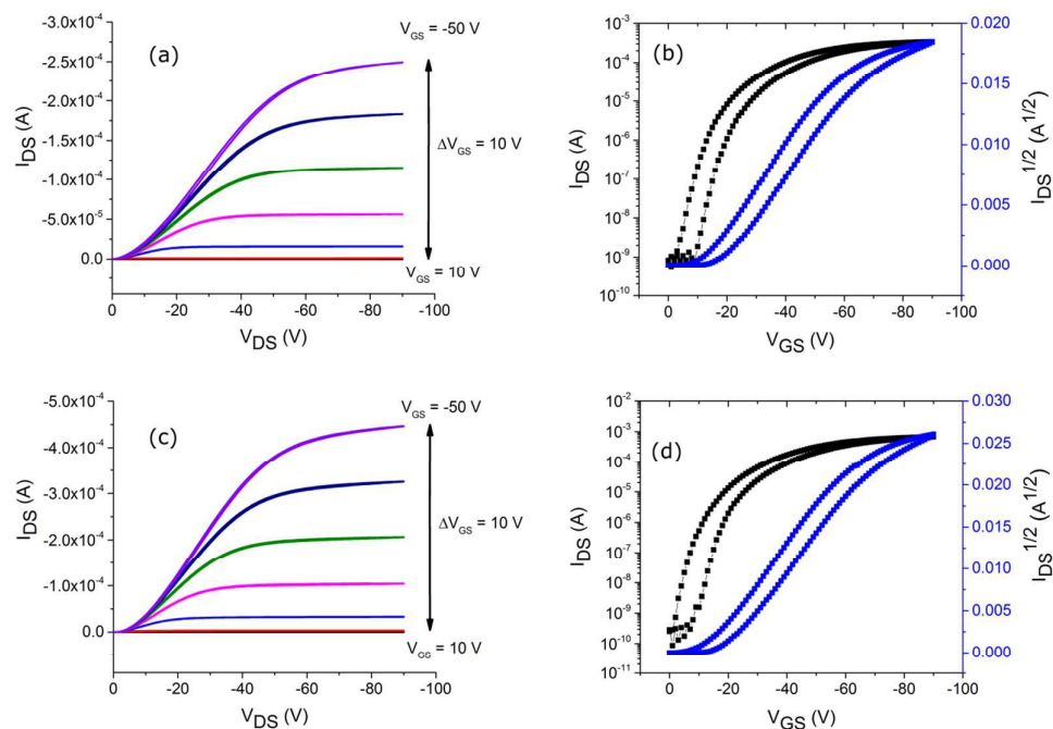
Figure 4: (a) and (b) show the output and transfer characteristics for an OFET fabricated using 5T-TTF; (c) and (d) are the output and transfer characteristics for an OFET fabricated with 5T-TTF + 5% CZTS.
