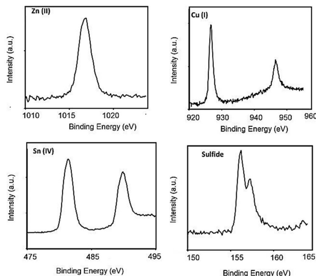
Figure 3: High resolution XPS spectra of CZTS nanoparticles synthesised at 220°C.
