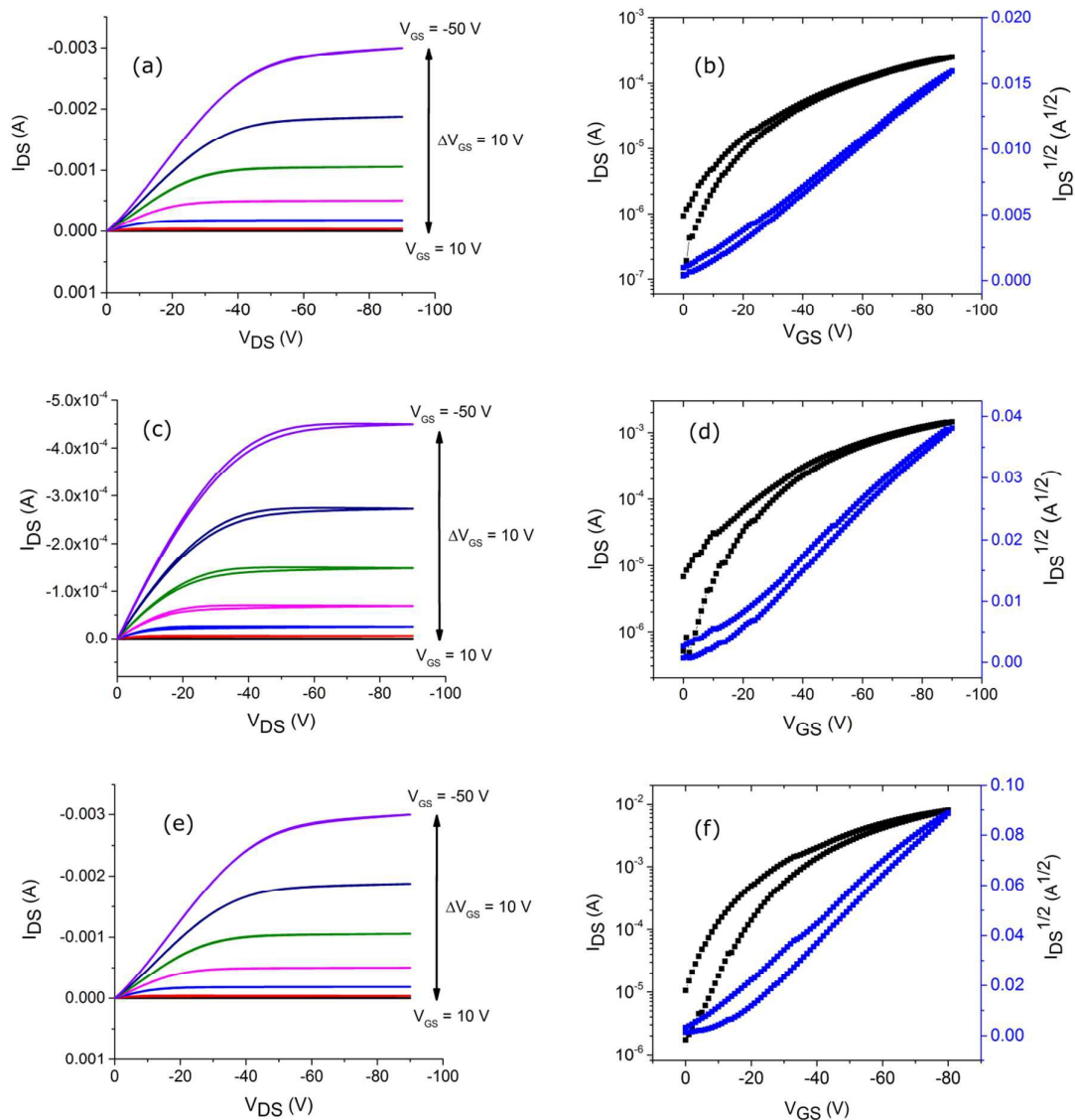
Figure 6: Output and transfer characteristics (left and right columns, respectively), for OFETs fabricated using neat P3HT [(a) and (b)], P3HT + 5% CZTS [(c) and (d)], and P3HT + 10% CZTS [(e) and (f)].
