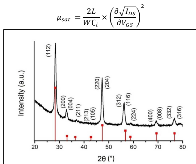
Figure 1: The p-XRD patterns of CZTS nanoparticles synthesised at 220°C for 1 hour. The reference patterns are of kesterite CZTS (ICDD: 04-015-0223). The TEM images showed hexagonal particles with an average size of 10 \pm 2 nm. The high resolution TEM (HRTEM) images shown in Fig. 2a and 2b, exhibit clear lattice fringes with measured d-spacing of ca. 0.313(1) nm corresponding to the (112) lattice plane of the kesteritic CZTS structure (Fig. 2c). The elemental composition of the CZTS nanocrystals was determined by energy dispersive X-ray spectroscopy (EDX), which gave a Cu/Zn/Sn/S composition (atomic %) of Cu (28.43%), Zn (11.38%), Sn (12.85%) and S (47.34%).
