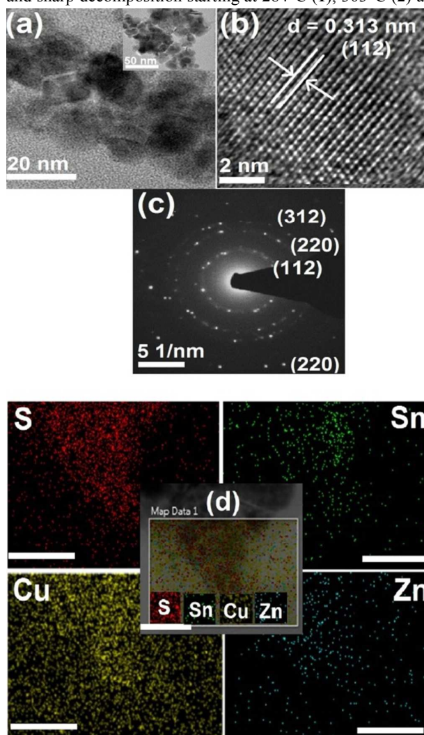
Figure 2: (a) and (b) are the HRTEM images, (c) the diffraction patterns and (d) the elemental map of CZTS nanoparticles synthesised at 220°C. The scale bar shown for the elemental map is ca. 50 nm.
