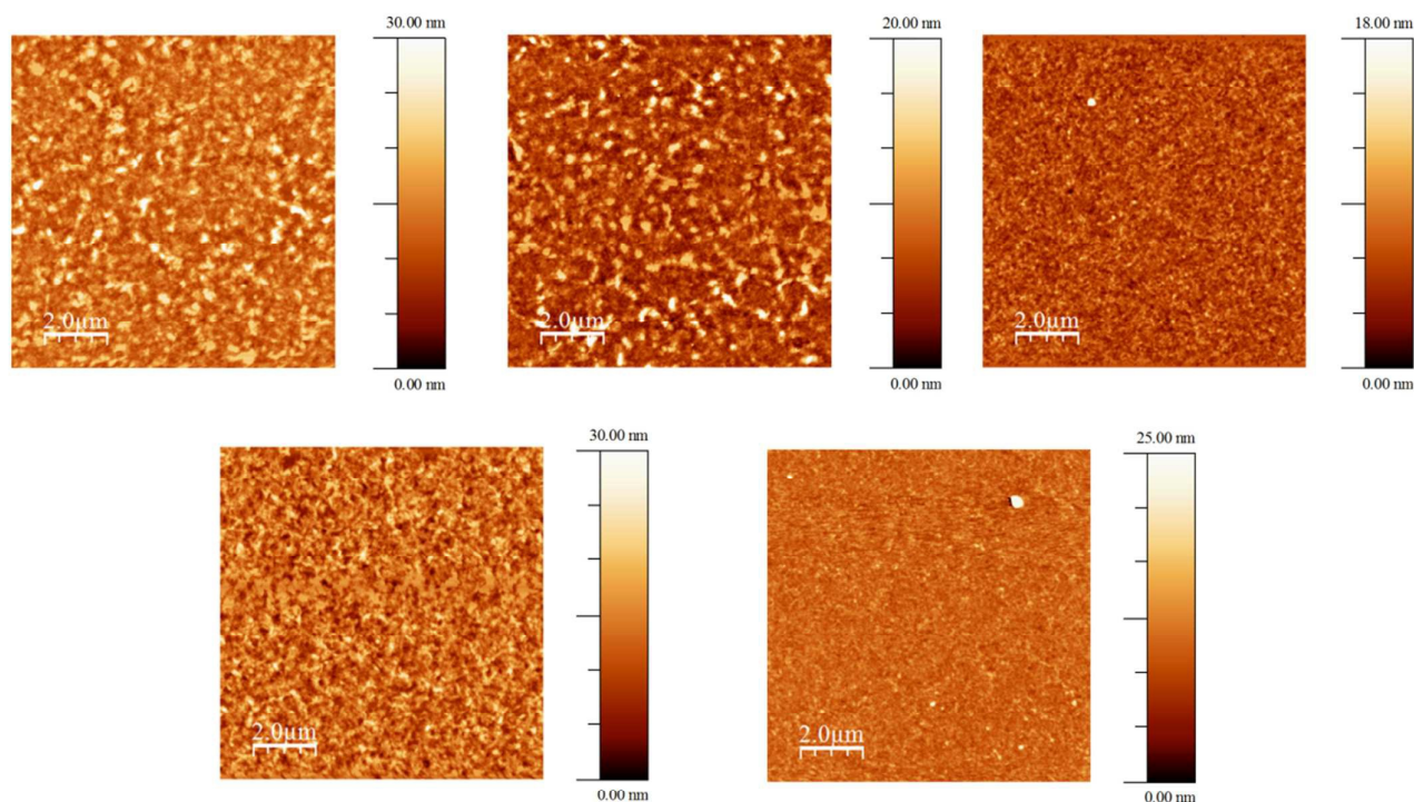
Figure 7: AFM images for OFETs fabricated using P3HT (top, left), P3HT + 5% CZTS (top, centre), P3HT + 10% CZTS (top, right), P3HT + 15% CZTS (bottom, left) and P3HT + 20% CZTS (bottom, right).
