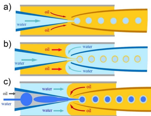
4 Fig. 3 Schematic illustration of the coaxial capillary microfluidic devices for generation of a) single (W/O), b) double (W/O/W) and c) triple (W/O/W/O) emulsions.
