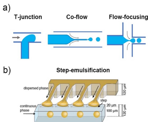
Fig. 1 a) Schematic illustration of various channel geometries including cross-flow, co-flow, and flow-focusing. b) Schematic illustration of a step-emulsification channel arranged with four parallelized drop markers. 33 The drop breakup occurs at the step between the nozzle and the continuous phase channel. Reprinted with permission from ref. 33. Copyright 2016, John Wiley & Sons, Inc.
