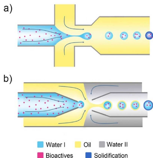
Fig. 10 Encapsulation of bioactives, such as drugs, proteins, and cells, a) in microspheres/microgels templated with single emulsions generated from a PDMS device and b) in the liquid core of microcapsules templated with double emulsions generated from a glass capillary device.
