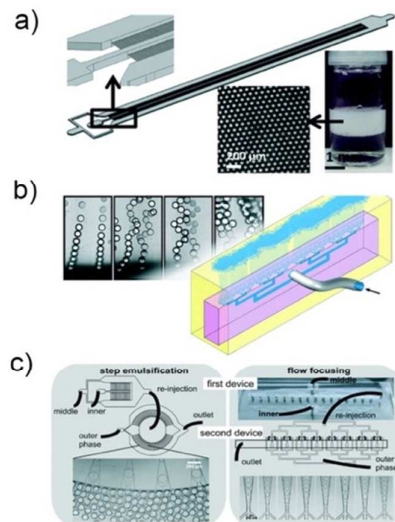
Fig. 2 a) Schematic illustration of the millipede device 36 and the drops produced. Reprinted with permission from ref. 36. Copyright 2016, The Royal Society of Chemistry. b) Droplet clearance from the nozzle exits in PDMS volcano device. 42 Reprinted with permission from ref. 42. Copyright 2018, The Royal Society of Chemistry. c) Schematic illustration of tandem emulsification. 43 Reprinted with permission from ref. 43. Copyright 2017, The Royal Society of Chemistry.
