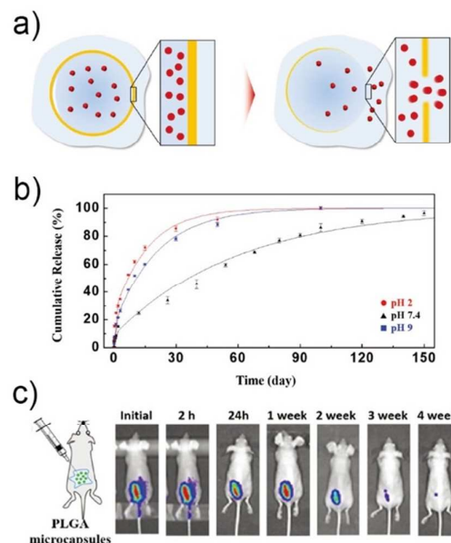
Fig. 14 a) Schematic illustration of release of encapsulants through a hole formed at the thinnest part of a PLGA membrane by degradation, 145 b) Cumulative release of sulforhodamine B from the microcapsules at different pH. c) In vivo fluorescence images for ICG-loaded PLGA microcapsules that are subcutaneously injected into dorsum of mice. Reprinted with permission from ref. 145. Copyright 2017, John Wiley & Sons, Inc.
