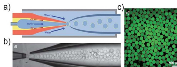
Fig. 4 a) Schematic illustration of the microfluidic device for preparation of double-emulsion droplets with an ultra-thin shell. 49 b) Optical microscope image showing the continuous generation of double emulsion in dripping mode. c) Confocal microscope images of microcapsules with a poly(lactic acid) membrane. Reprinted with permission from ref. 49. Copyright 2011, The Royal Society of Chemistry.
