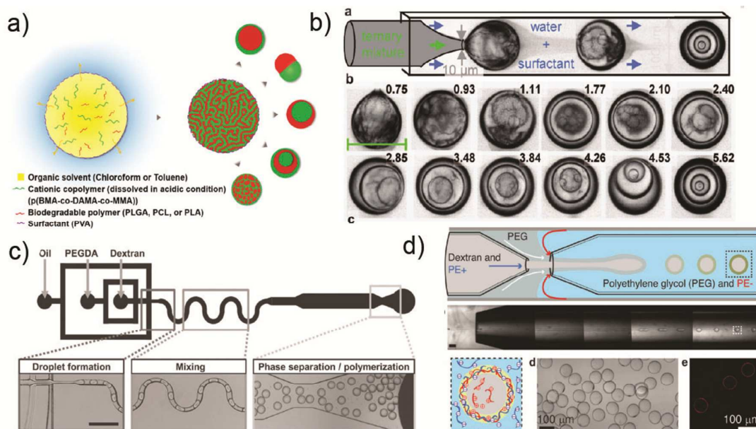
Fig. 7 Other methods utilized in converting emulsion droplets to solid microparticles. a) Formation of microparticles with various configuration through phase separation in emulsion drops. 98 Reprinted with permission from ref. 98. Copyright 2016, American Chemical Society. b) Formation of quintuple emulsion drops from single emulsion drops via phase separation. 95 Reprinted with permission from ref. 95. Copyright 2014, John Wiley & Sons, Inc. c) Synthesis of dextran/PEG microparticles by utilizing ATPs. 109 Reprinted with permission from ref. 109. Copyright 2012, John Wiley & Sons, Inc. d) Fabrication of microparticles through interpolymer complexation between polyelectrolytes in ATPs. 113 Reprinted with permission from ref. 113. Copyright 2016, John Wiley & Sons, Inc.
