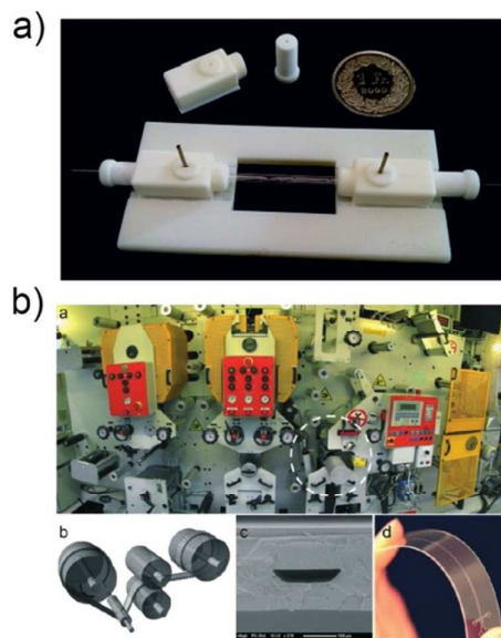
Fig. 5 a) A 3D-printed assembly of capillary device ready for use. 68 Reprinted with permission from ref. 68. Copyright 2014, The Royal Society of Chemistry. b) Roll-to-roll hot embossing of microfluidic chips. 75 Reprinted with permission from ref. 75. Copyright 2016, The Royal Society of Chemistry.
