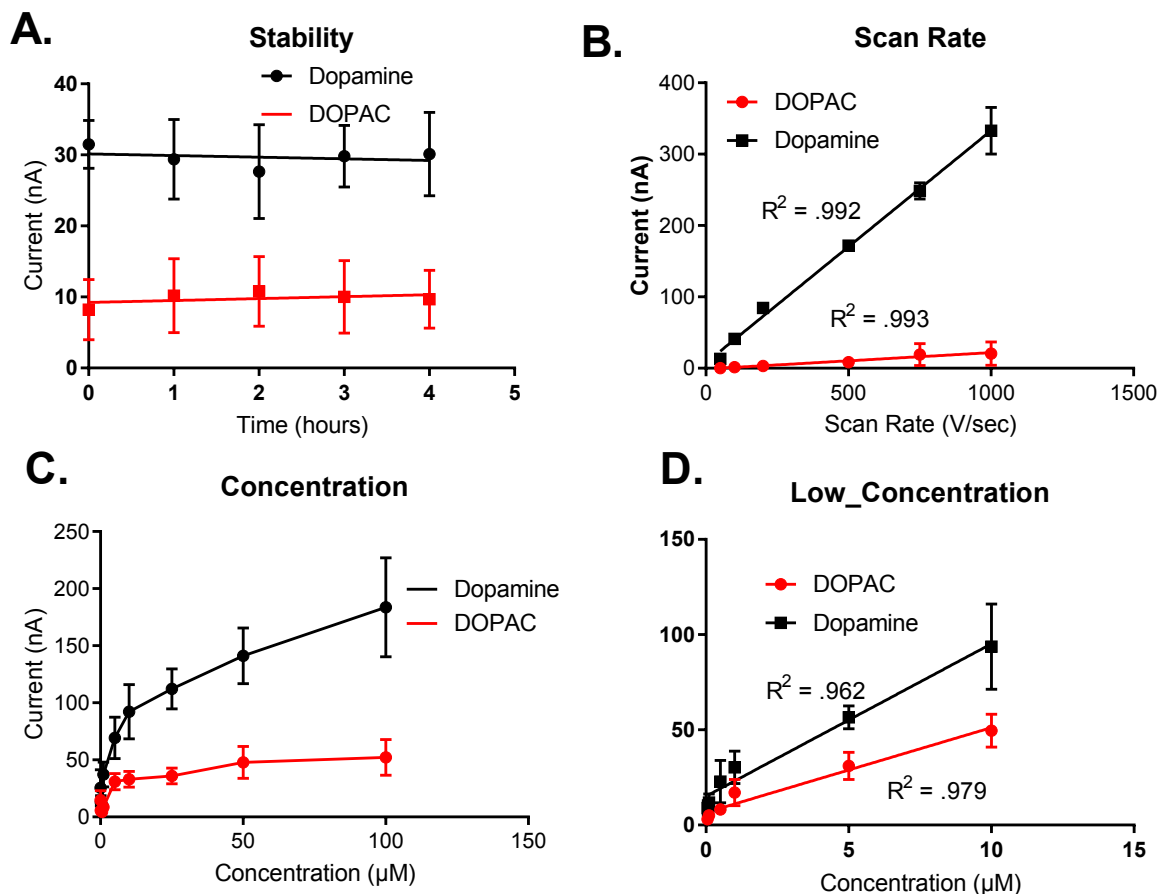
Figure 6. Adsorption Control Testing of the DOPAC waveform applied to Uncoated CFMEs. 6A.
