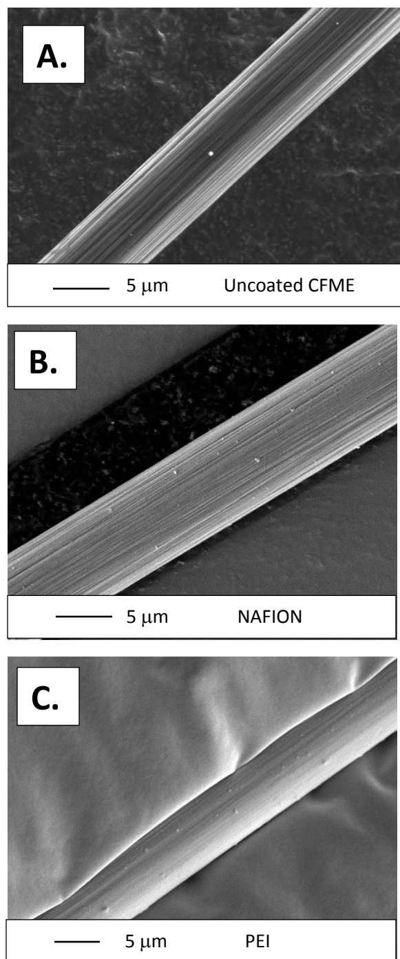
Figure 2: SEM Images of A). A bare uncoated carbon fiber approximately 7 microns in diameter. B). A carbon fiber electrodeposited in a Nafion solution for approximately 5 minutes. A thin layer of polymer evenly coats the surface of the electrode. C). Polyethyleneimine (PEI) Coated Carbon fibers. The disappearance of the ridges in Figures 2B and 2C indicate that the carbon fibers have been coated in a thin layer of polymer. Small dots on the surface of the fibers are remnants of gold sputtering that were utilized to increase the conductivity, and hence resolution, of the images.
