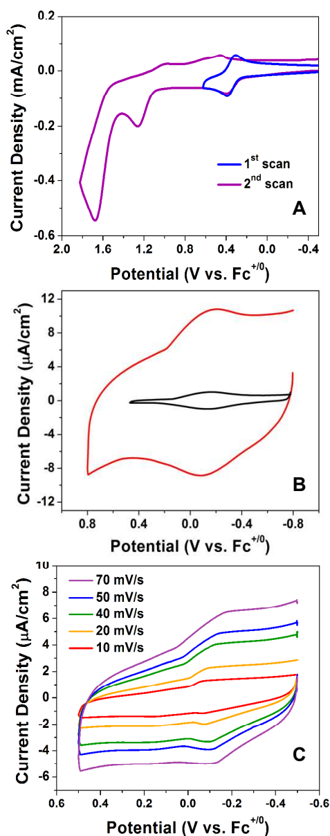
Figure 2. CV of [Ni(propargyl-cyclam)] 2+ in 0.1 M TBAPF 6 /DCM solution. Scan rate 100 mV/s (A). CV of mod-GCE-1 in 0.1 M TBAPF 6 in DCM. Scan rate 100 mV/s (red), 5 mV/s (black) (B). CV of mod-GCE-1 in 0.1 M TBAPF 6 in DCM at various scan rates (C).
