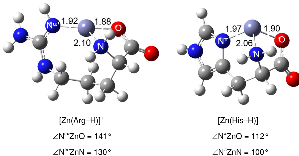
Fig. 6 Comparison of [\text{Zn}(\text{Arg-H})]^+ and [\text{Zn}(\text{His-H})]^+ ground structures. 22 Bond lengths (in Å) are indicated for select bonds.
