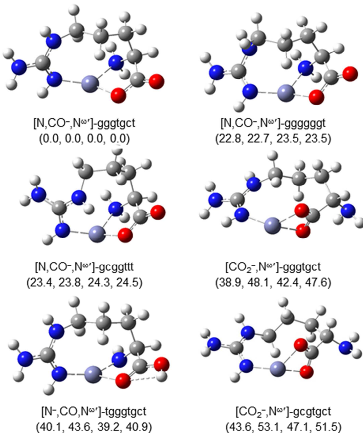
Fig. 1 Structures of low energy [Zn(Arg-H)] + conformers calculated at the B3LYP/6-311+G(d,p) level of theory. Relative 0 K enthalpies (kJ/mol) are given at the B3LYP, B3LYP-GD3BJ,
