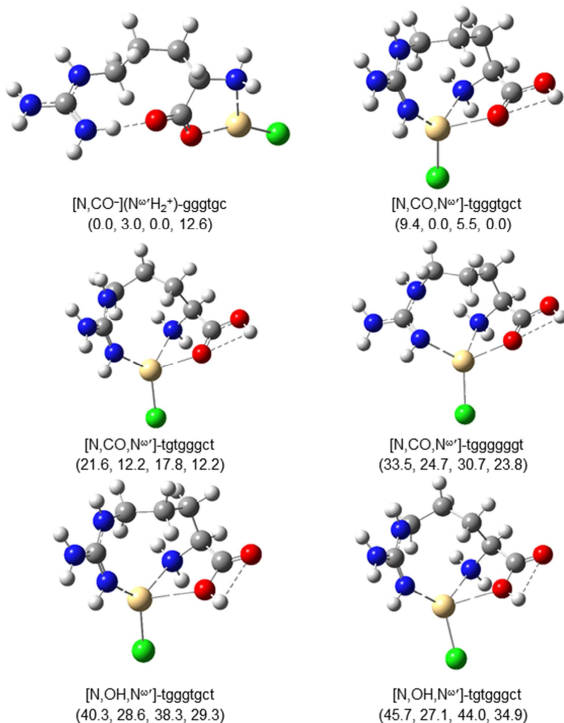
Fig. 2 Structures of low energy CdCl + (Arg) conformers calculated at the B3LYP/def2-TZVP level of theory. Relative 0 K enthalpies (kJ/mol) are given at the B3LYP, B3LYP-GD3BJ, B3P86, and MP2(full) levels, respectively. Short dashed lines indicate hydrogen bonds and long dashed lines indicate Cd-ligand bonds.
