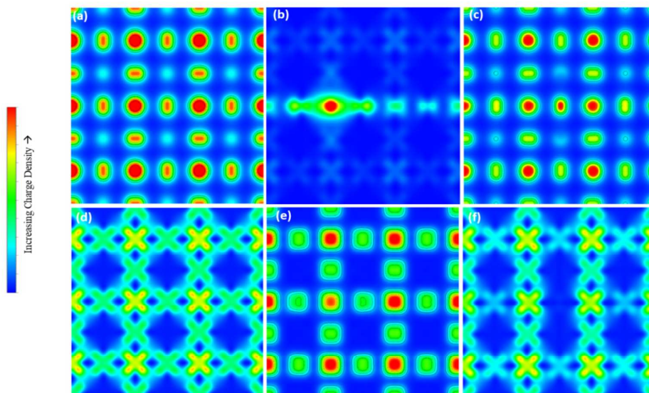
Fig. 2 Partial charge density calculations for pristine anatase TiO 2 (a & d), anatase TiO 2 with O vacancy (b & e), anatase TiO 2 with Ti vacancy (c & f). Images a-c refer to the valence bands, d-f are the conduction bands. 2D images projected along the c axis.
