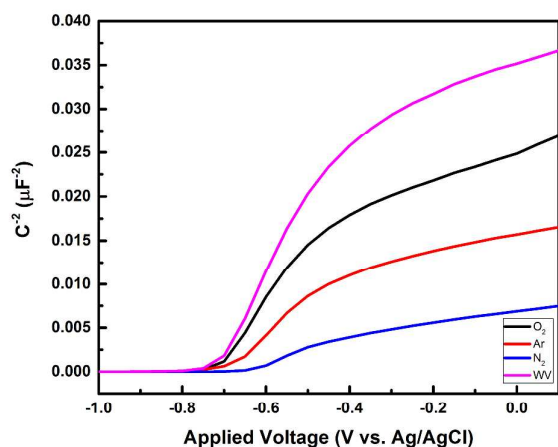
Fig. 3 Mott-Schottky plots at 1.3 kHz of anatase TiO 2 nanotubes annealed under different atmospheres.
