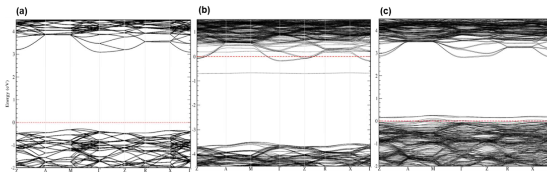
Fig. 1 Theoretical band structures of a) pristine anatase \text{TiO}_2 , b) anatase \text{TiO}_2 with O vacancy, and c) anatase \text{TiO}_2 with Ti vacancy stabilized with 4 protonated O sites. Red line indicates the Fermi energy.
