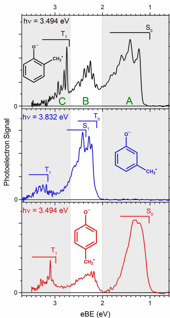
Fig. 3 Photoelectron spectra of the m/z = 106 anions produced from reaction of O^- with three isomers of methylphenol. Spectra were taken with the pulsed PES instrument with a photon energy of 3.494 eV or 3.832 eV. The spectra are highlighted to differentiate three regions, labelled A, B, and C. The inset methylenephenoxide anion structure shows the primary isomer anion responsible for the observed PES in regions A and C (for ortho and para ) and region B and C ( meta ). The electronic states of the dominant neutral molecules accessed from electron photodetachment of the methylenephenoxide anion are also labeled.
