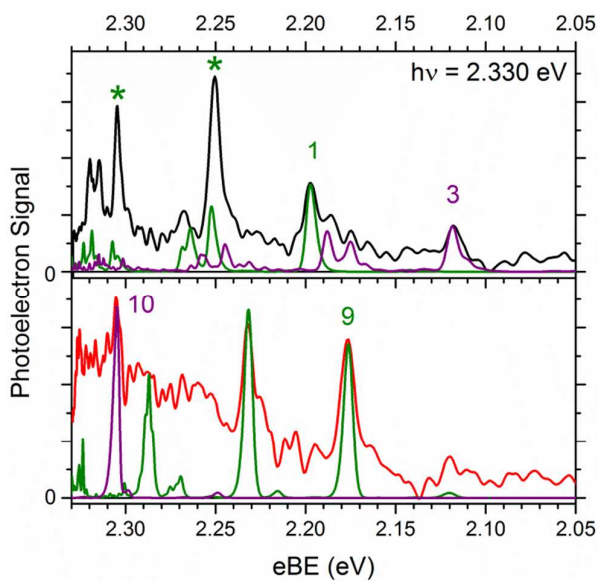
Fig. 6 Photoelectron spectra of m/z = 106 , resulting from the reaction of O^- with o - (black) and p - (red) methylphenol, collected with the pulsed PES instrument with a photon energy of 2.330 eV. The numeric labels indicate the isomer listed in Fig. 2, and the asterisks are discussed in the text. The simulated PES, following their convolution with the experimental resolution, are shown in green and purple lines. The calculated transitions and their corresponding FCFs are shown in the ESI.
