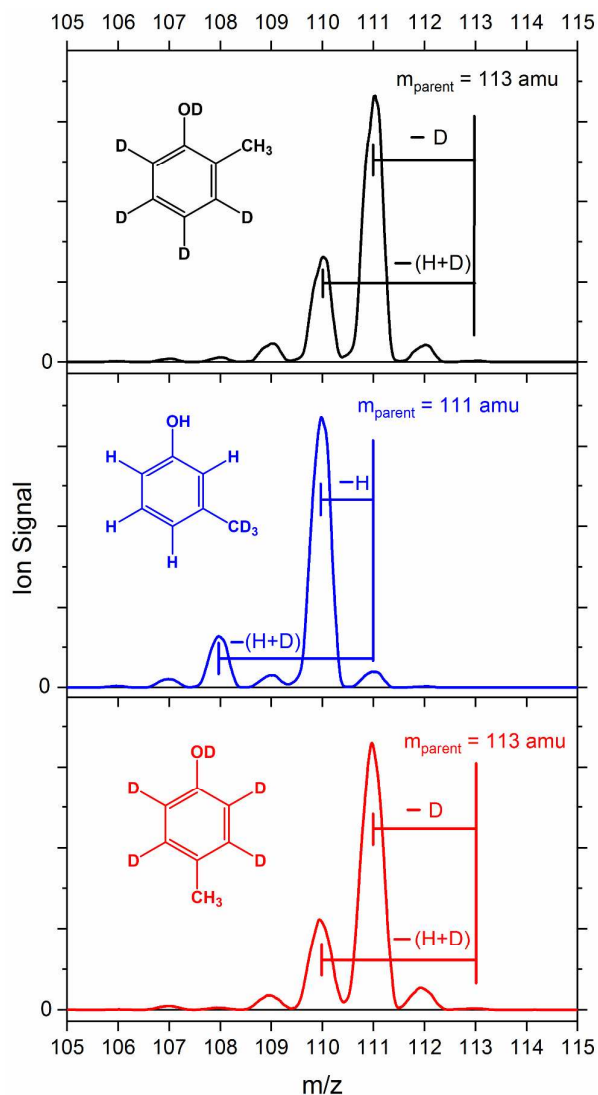
Fig. 1 Mass spectra collected with the FA-SIFT instrument of selectively deuterated o - (black), m - (blue), and p - (red) cresols reacted with O^- . In each panel, the parent cresol structure is shown and a vertical line indicates the parent mass. For each isomer, deprotonation from the O site is the largest observed product channel, while the next largest channel is (H + D) loss from the hydroxyl and methyl groups. More details may be found in the text.
