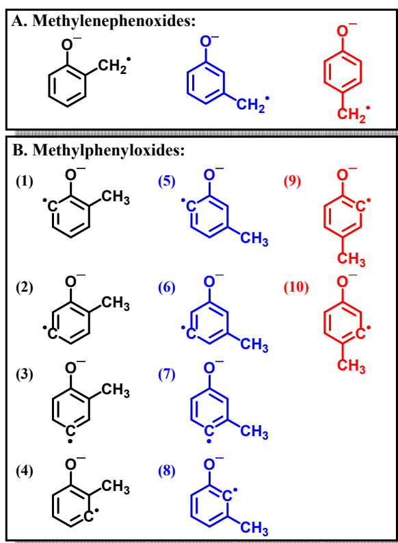
Fig. 2: Possible anion isomers, based on results from isotope studies (Fig. 1) and thermodynamic calculations, formed following the reaction of O^- with o - (black), m - (blue), and p - (red) methylphenol, resulting in the abstraction of (H + H^+) . The anions are split into two categories: methylenephenoxides (panel A) and methylphenyloxides (panel B).
