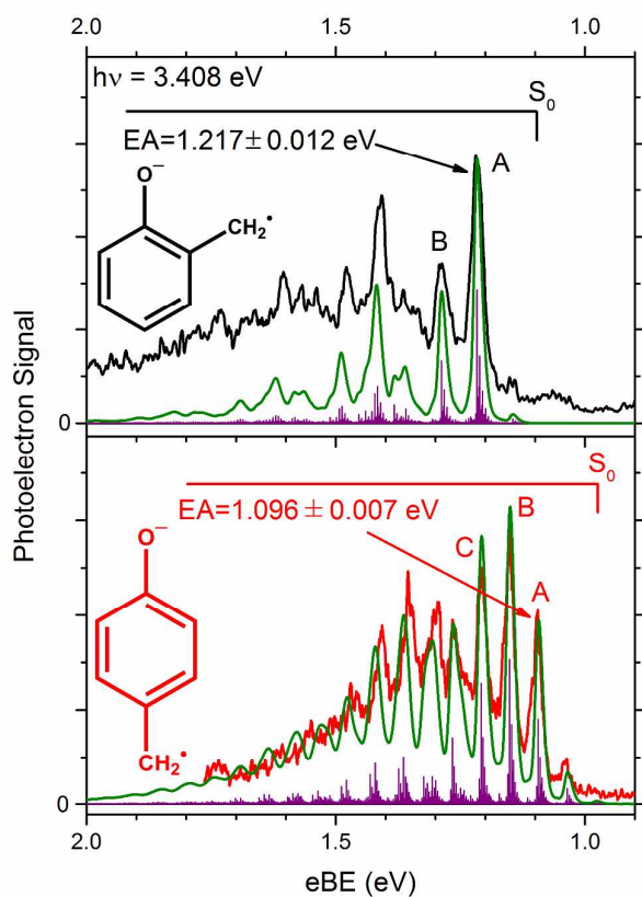
Fig. 4 Photoelectron spectra of the o - and p -methylenephenoxide anions obtained with the continuous PES instrument utilizing a photon energy of 3.408 eV are shown in the black and red traces, respectively. This instrument has a constant spectral resolution of 10 meV. The calculated transitions and their corresponding Franck–Condon intensities are represented by purple sticks, while their convolution with experimental resolution are shown in green.
