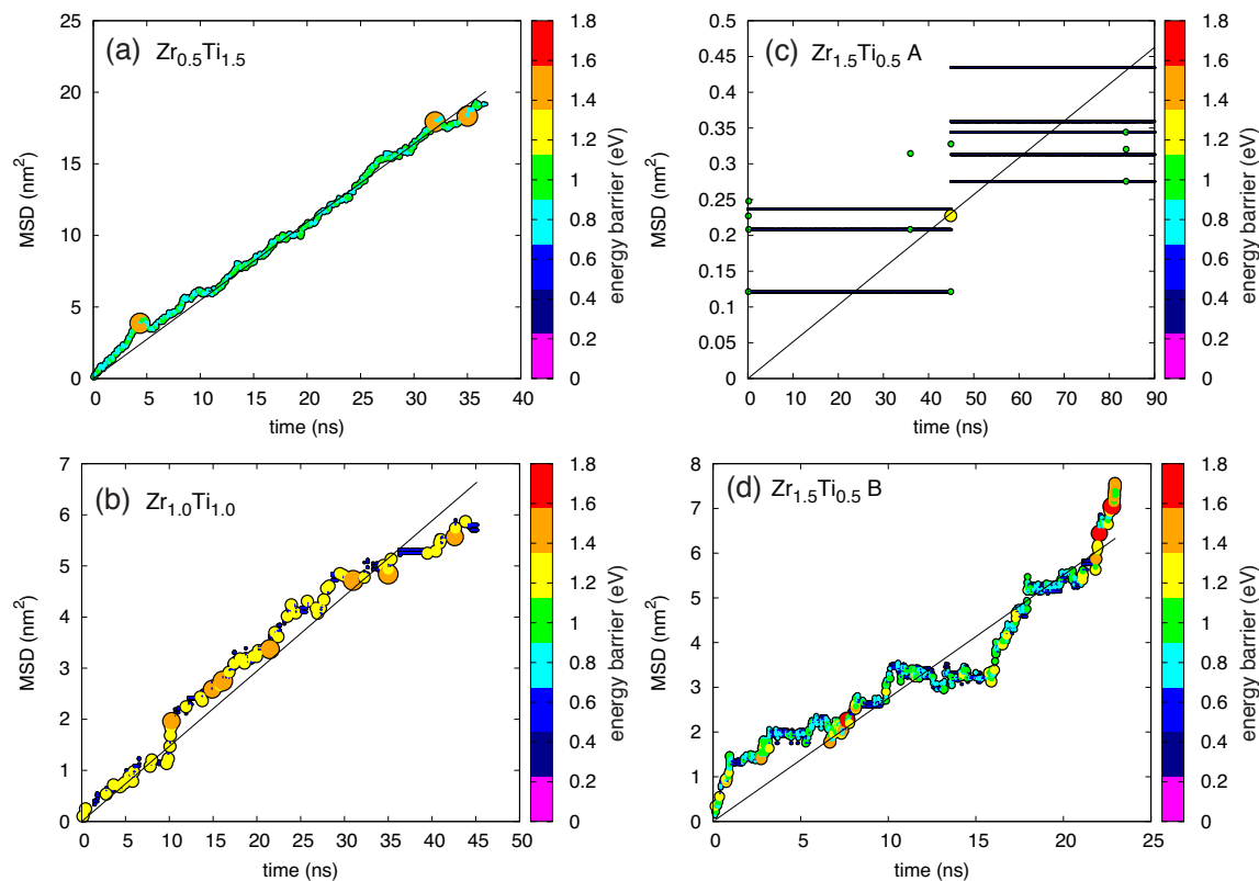
Fig. 7 The MSD of the atoms versus times in the four simulations described above. All MSDs are referenced to t = 0\text{ns} . The points represent the time at which an event occurred and both the size and the color scale with the absolute energy of the barrier describing that event (with the relationship size/color energy 3 , for clarity). The lines are linear fits to the MSD, the slope of which gives 2D , with D being the diffusivity of the atoms during the course of the simulation. When the barriers are particularly small, they only appear as small dots in the figures. This is particularly evident in (c), where the overlapping barriers appear as horizontal lines.
