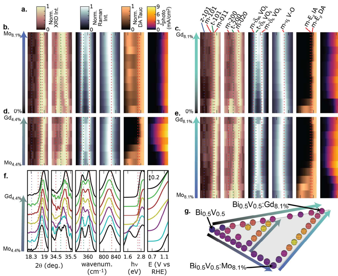
Figure 4. (a.) Combinatorial characterization of Bi-V-Mo-Gd alloys where a. provides the color scale for the normalized XRD, Raman, and UV-vis (Tauc) signals as well as the PEC ( J_{photo} ) signal; (b.-e.) contain false color plots for 4 different composition lines; (f.) is the stack-plot representations of the data from d. and also provides the labels for the horizontal axes, where the portions of each signal are chosen to highlight pertinent features; c. provides the labels for select literature values shown as dashed lines in each respective plot; and g. provides the visualization of the 4 composition lines, which are all in the x = 0.5 plane of Figure 2d. False color plots shown for all 4 composition lines aid visual recognition of trends among the 4 composition lines. The descriptions of the dashed lines are as follows: z-101 is the {101} XRD peak for the zircon polytype and is a distinguishing peak to confirm that this polytype is not observed in any substantial phase fraction. The tetragonal scheelite ("t") {101} and {200} XRD peaks split to {101} and {011} and to {200} and {020} peaks for the monoclinic (distorted scheelite) phase ("m"). Similarly the VO 4 bending mode ( \delta_s ) in t-BiVO 4 splits into asymmetric ( \delta_{as} ) and symmetric ( \delta_s ) modes in m-BiVO 4 . The alloying-driven lessening of the monoclinic distortion results in merging of each of the monoclinic doublet peaks, and the \delta_{as} and \delta_s peaks provide the best resolution of the monoclinic distortion and reveal that none of these materials have tetragonal symmetry. The symmetric V-O bending mode ( \nu_s ) is also shown at the value for m-BiVO 4 . The literature positions of the indirect (IA) and direct (DA) allowed band gaps of m-BiVO 4 are shown with each composition showing a strong increase in DA Tauc signal in this energy range and many compositions exhibiting substantial sub-gap absorption that is modulated in both intensity and characteristic photon energy through alloying. Each J_{photo} signal is the fitted curve to the chopped-illumination anodic voltage sweep and as the only non-normalized type of signal in the figure, a 0.2 mA cm -2 scale bar is shown in f.
