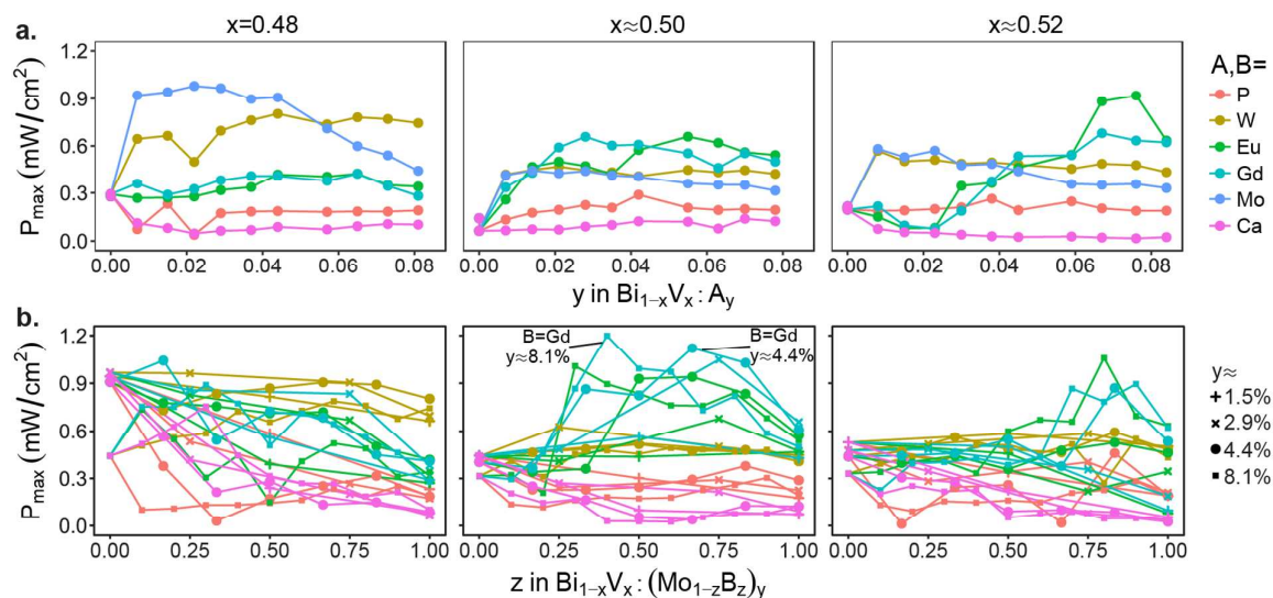
Figure 3. (a.) The P_{\max} variation with alloy loading for each Bi-V-A system reveals Mo and W as the best elements with x = 0.48 (Bi-rich) and Gd and Eu with x = 0.52 (V-rich) compositions. (b.) The co-alloying in Bi-V-Mo-B spaces for 5 values of B, each of which includes 4 different total alloy loadings ( y ) shown as different symbols. Each segmented line spans Bi-V-Mo ( z=0 ) to Bi-V-B ( z=1 ) at the specified loading, with a linear or convex trends expected for Mo-B combinations that do not improve performance beyond the respective alloying sub-spaces. For Mo-Gd with x = 0.5 , the trends for all 4 loadings are concave with the 2 labelled curves containing the highest P_{\max} values. The relative uncertainty in P_{\max} for each data point is estimated to be 13%, and for clarity is not illustrated.
