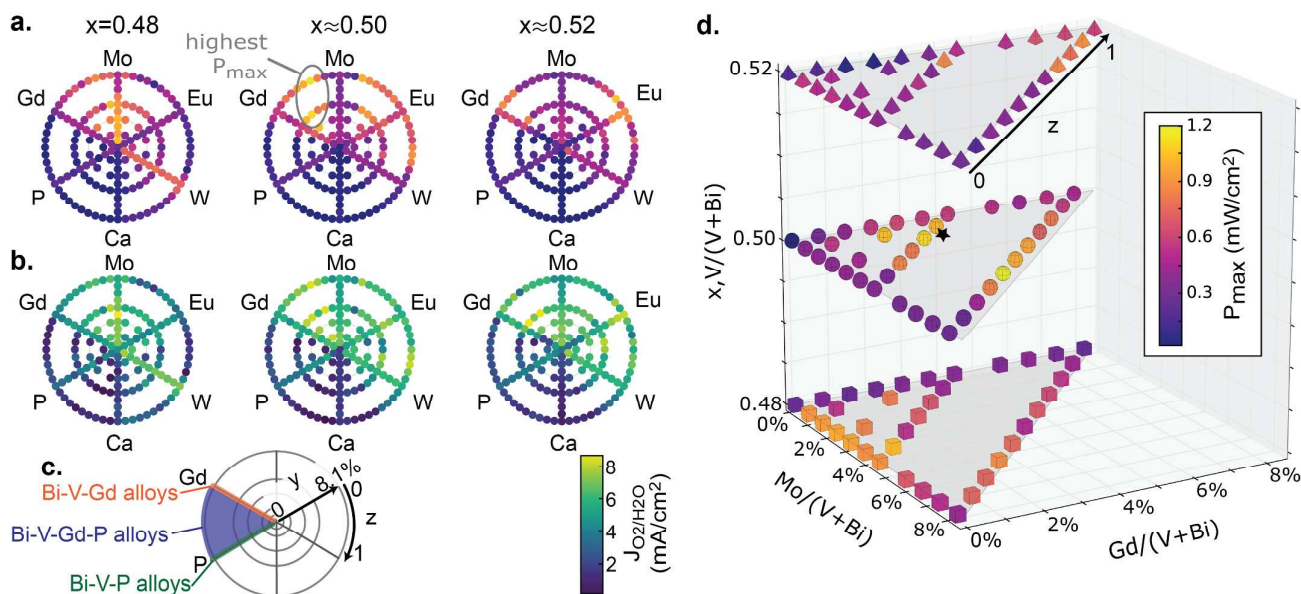
Figure 2. (a.) P_{\text{max}} values for 489 of the 948 unique compositions in the photoanode library. In this series of radial plots for each x value, the \text{Bi}_{1-x}\text{V}_x composition is at the center with the 6 radial lines corresponding to Bi-V-A alloys and the 6 sectors containing Bi-V-A-B alloys. The 9 Bi-V-A-B composition spaces not represented in the 6-sector plots comprise the remainder of the library compositions. (b.) The analogous map of J_{\text{O}_2/\text{H}_2\text{O}} values from the same anodic sweep dataset, which upon comparison with the P_{\text{max}} map reveals somewhat different compositional trends and indicates the importance of specifying a figure of merit to identify an optimal alloy. (c.) Legend for the radial alloy loading ( y ) and azimuthal alloy-composition ( z ) variables. (d.) The Mo-Gd sectors from a. are plotted in Cartesian space where the three x values correspond to the 3 highlighted planes, and the black star denotes the Bi-V-Mo-Gd composition used for scale-up studies. The P_{\text{max}} color scale is the same for a. and d. and is also the same as Figure 1c.
