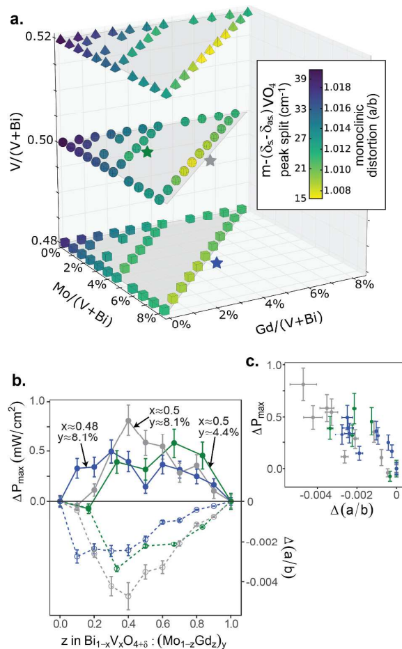
Figure 5. (a.) Map of the level of splitting of the asymmetric ( \delta_{as} ) and symmetric ( \delta_s ) VO_4 bending modes from Raman characterization of Bi-V-Mo-Gd alloys. The false color scale is also annotated with the monoclinic distortion inferred from the Raman peak splitting using Eq. 2. (b.) For the 3 composition lines marked by stars in a., both P_{max} and monoclinic distortion are plotted as deviations ( \Delta ) from the linear interpolation between the respective endpoint Bi-V-Mo and Bi-V-Gd compositions. (c.) The left-y and right-y axis data from b. are plotted to highlight the strong correlation between the decrease in monoclinic distortion below the Vegard law expectation and the co-alloying enhancement of P_{max} . The Pearson correlation coefficient of these data is -0.83.
