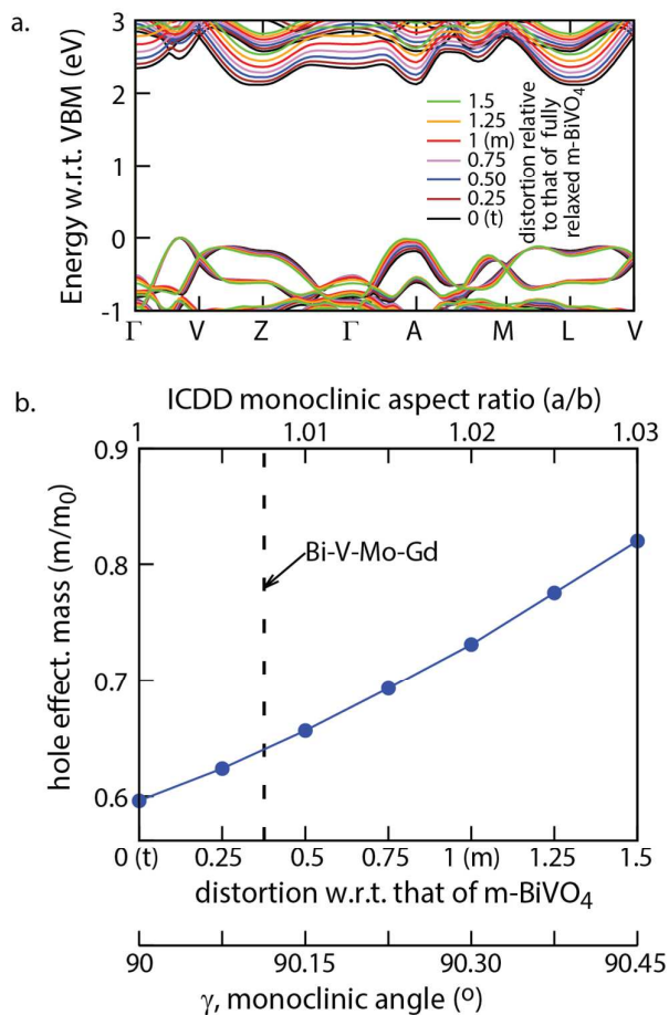
Figure 6. (a.) Computed band structure (DFT-GGA) for a series of crystal structures including the high-symmetry, DFT-HSE fully-relaxed tetragonal (0, t-BiVO 4 ), the low-symmetry DFT-HSE fully-relaxed monoclinic (1, m-BiVO 4 ) to 5 additional structures with the noted magnitude of monoclinic distortion. (b.) Hole effective mass at the \Gamma -V VBM for the 7 structures. The upper axis shows the monoclinic ratio (a/b) for comparison with experimental values in Figure 5, and the monoclinic ratio of the Bi-V-Mo-Gd alloy with highest P_{\max} is shown with a dotted line.
