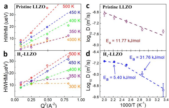
Figure 4. Variation of HWHM with Q^2 for different temperatures of LLZO a and H_x -LLZO b . The dashed lines represent fits of \text{HWHM} = DQ^2 + c , where D is the diffusion coefficient. Temperature dependence of the diffusion coefficient for c LLZO and d H_x -LLZO, respectively. There are two segments of the plot for H_x -LLZO that indicates a different diffusion mechanism at a higher temperature. Some of the error bars are smaller than the symbols.
