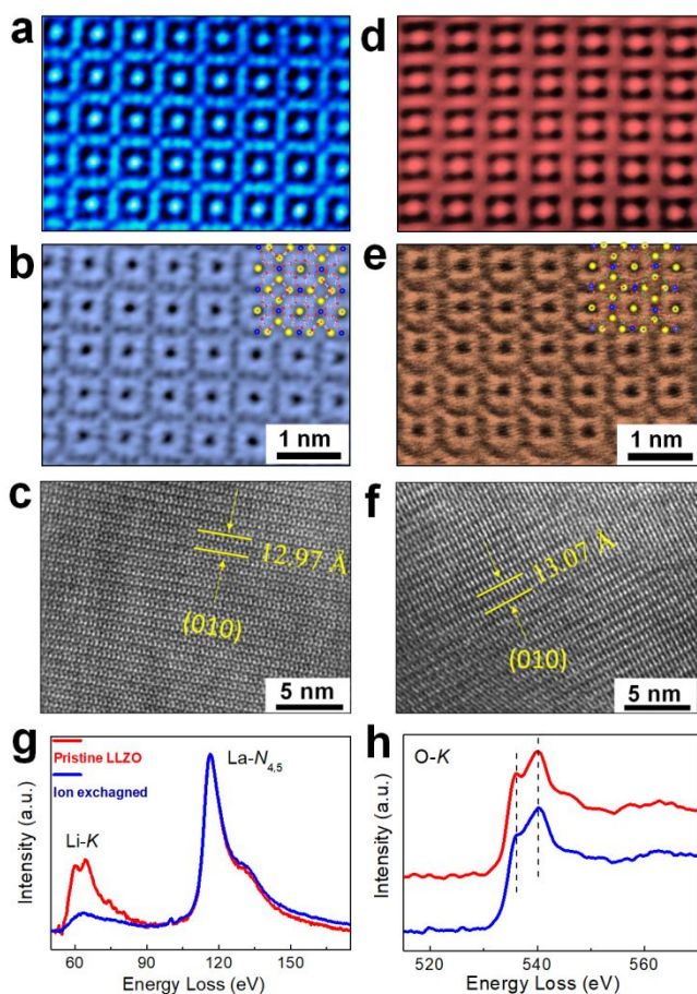
Figure 1. HAADF-STEM a , BF-STEM b , and HRTEM c images of pristine LLZO. The overlay in b is the schematic model with la-3d symmetry with a lattice
