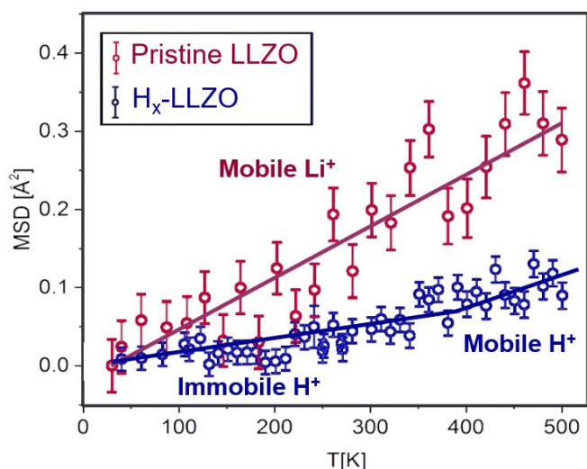
Figure 3. The average mean-square-displacement for LLZO and H_x -LLZO samples. H has a larger neutron cross-section which yields a 90% of signal when coexists with Li. Li dominates the incoherent neutron scattering signal of pristine-LLZO and furthermore, the other elements in the sample are not expected to undergo diffusive motions in the measured temperatures, thus the MSD in pristine-LLZO reflects Li dynamics. In contrast, the MSD of H_x -LLZO is mainly a reflection of H.
