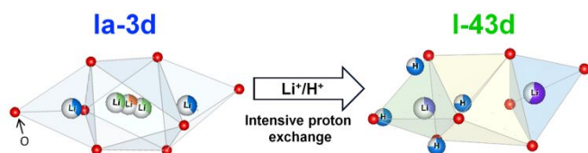
Figure 5. Schematic illustrations of structural and chemical modifications in c-LLZO after intensive proton exchange; the structure and ion occupancies of pristine 1a-3d LLZO are delineated based on previous reports. 42,43 Those for 1-43d LLZO are shown based on current work, e.g. Fig. 2 and Table S1.
