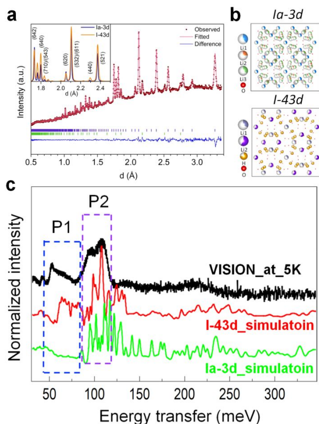
Figure 2. a Neutron diffraction of protonated LLZO powders. The dots are the experimental data, while the red line through them is the calculated model. The series of tick marks on the top represents the H_x -LLZO, and the tick marks on the bottom indicate coexisting LiOH ( 7.6 \pm 2.0 wt%). The bottom curves show the difference between the experimental data and calculated patterns. The inset shows the comparison of the fitted diffraction patterns of LLZO ( la-3d ) and H_x -LLZO ( l-43d ). Data extracted from this fit are given in Table 1. b Schematic configurations of la-3d and l-43d of H_x -LLZO. c Comparison between the experimental and calculated VISION-INS (inelastic neutron spectra) of H_x -LLZO with l-43d or la-3d structure. P1 and P2 are the marked peaks that show an obvious difference between l-43d and la-3d structure.
