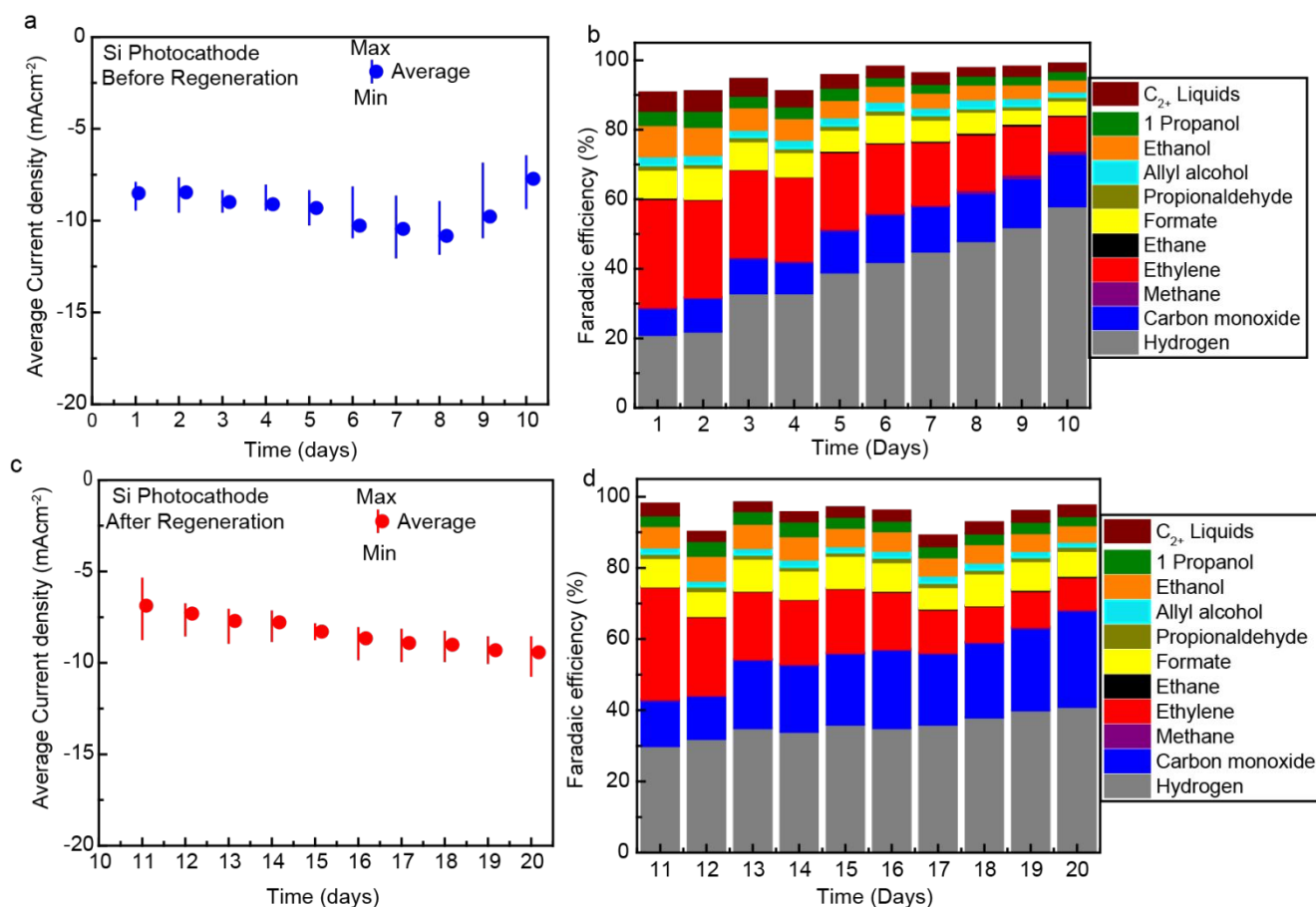
Fig. 4. Stability measurement of a textured silicon photocathode with an integrated Ag-supported dendritic Ag catalyst at -0.4 V vs RHE in 0.1 \text{ M CsHCO}_3 electrolyte solution under simulated 1-sun illumination. Simulated diurnal cycling was performed with 10 hrs light on and 14 hrs light off. The electrolyte was changed after each daily measurement of the liquid products. a. Daily average photocurrent over 10 days of the Si photocathode before regeneration of the catalyst. Current density data points were averaged over a day; the vertical line indicates the maximum and minimum current density on that day. b. \text{CO}_2\text{R} product distribution with time. c. Daily average/high/low photocurrent of the Si photocathode after Cu catalyst regeneration. d. \text{CO}_2\text{R} product distribution with time of the regenerated photocathode.
