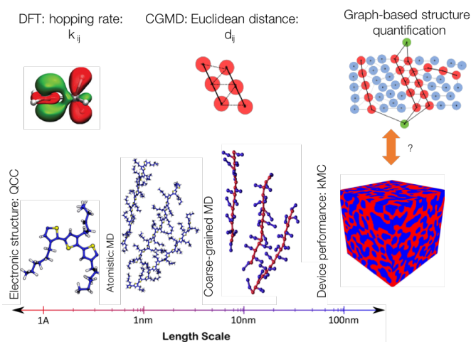
Fig. 1 This work combines hopping rates on sub-nanometer length scales with network connectivities over 100+ nanometers to infer the conditions needed for fast charge transport in organic electronic films. The bulk charge transport properties of an organic thin film depends on how the electronic orbitals of chromophores are locally oriented with respect to each other, the packing of polymer chains, and the connections between disparate nanostructured elements.
