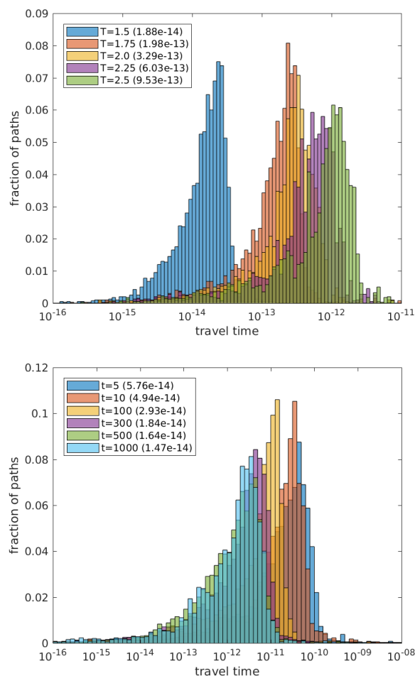
Fig. 10 Histogram of shortest path travel times for five equilibration temperatures (top), and six snapshots from the T = 1.5 equilibration. Note the two orders of magnitude difference in average travel time between T = 1.5 and T = 2.5 . The travel times of charges along the shortest paths from a vertex to the nearest boundary vertex correlate well with the mobility calculation from kinetic Monte Carlo calculations (Table 1).
