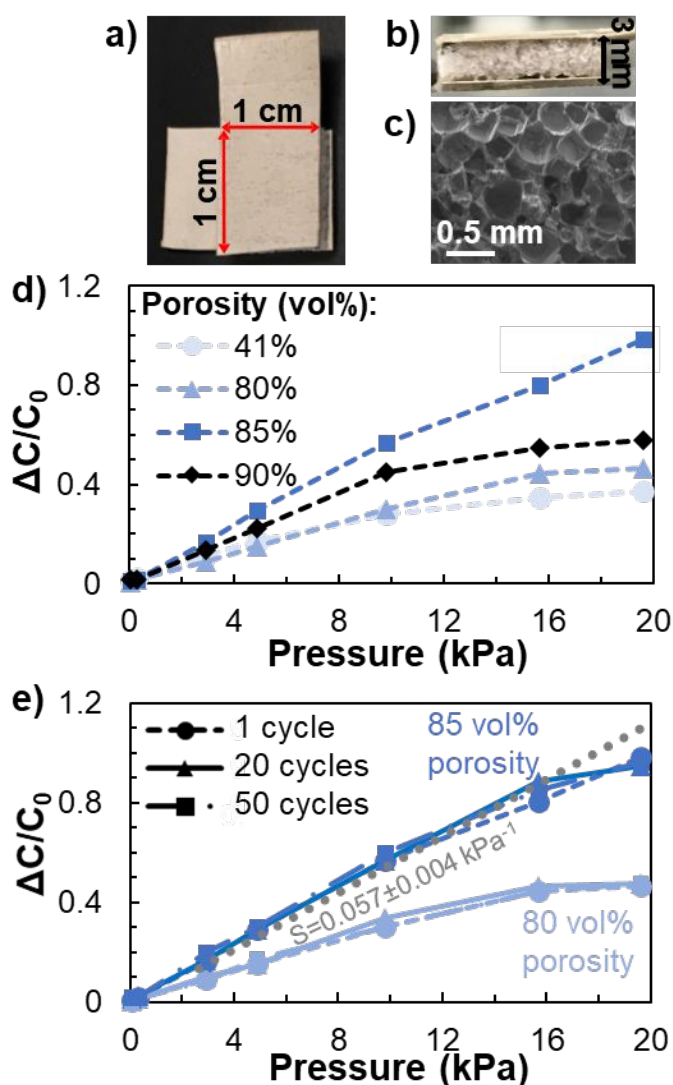
Figure 2. Pressure sensor characteristics. a) Top and b) side view of the capacitive pressure sensor. c) SEM micrograph of the porous dielectric. d) Relative capacitance change as function of the applied pressure. The porosity
