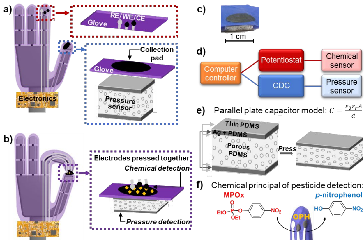
Figure 1. Dual-functionality glove design and principal operation mechanisms. a) The glove combines both pressure and chemical sensors. Reference (RE), working (WE), and counter (CE) electrodes are screen printed on one digit, and the collection pad is printed on a separate digit. b) The electrodes are pressed together to initiate the electrochemical analysis. c) The pressure sensor is below the glove substrate underneath the chemical sensor collection pad. d) System architecture. e) Pressure sensor is based on a parallel plate capacitor with porous PDMS dielectric and flexible electrodes. f) Chemical sensor detects the reaction product p-nitrophenol using three-electrode electrochemical techniques, including SWV and amperometry.
