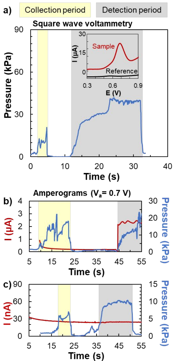
Figure 4. Simultaneous pressure and chemical detection. a) Pressure sensor measurement during the sample collection step (yellow region) and the chemical detection step (gray region). The electrochemical SWV scans in the inset were initiated when the collection pad was pressed and in good contact with the measurement electrodes, as indicated by the exceeding pressure. Same color schemes are used for collection and detection periods for plots b and c. Simultaneous measurements of pressure and amperogram at the applied potential of +0.7 V. The electrochemical sensor current increased for b) the tomato sample spiked with MPO x (200 µL at 200 µM concentration). The current did not change for c) the control tomato surface with no pesticide, while the pressure signal indicated that the collection pad and measurement electrodes are in good contact for proper electrical connections during the electrochemical measurements.
