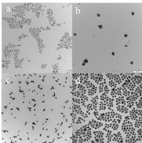
Fig. 4 TEM images of iron oxide (11 nm) before assembly (a) and after incorporation into ZnMONs (b), UCNP before (c) and after incorporation into ZnMONs (d). Scale bar: a 50 nm; b, c, and d 200 nm.
