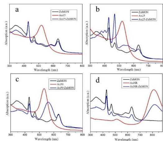
Fig. 2 UV-vis spectra of ZnMON, Au nanoparticles and corresponding Au nanoparticles incorporated into ZnMONs. (a) Au15 and Au15-ZnMONs, (b) Au25 and Au25-ZnMONs, (c) Au50 and Au50-ZnMONs, (d) AuNR and AuNR-ZnMONs.
