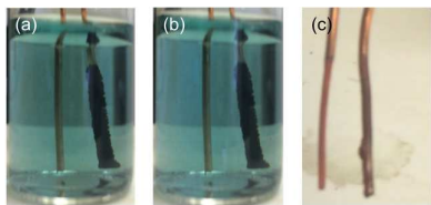
Fig. 9. Photographs of an experiment involving copper electrodes in with a-SWCNTs (0.0034 mg/mL) in a \text{CuSO}_4 solution ( 0.1 \text{ mol/dm}^3 ) before and after two time intervals of electrolysis: (a) 0 s, (b) 53 s, and (c) 879 s. The left electrode is the anode while the right electrode is the cathode.
