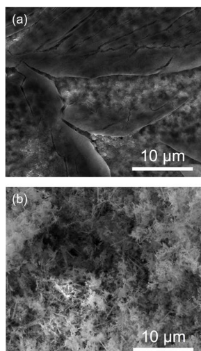
Fig. 10. SEM images of (a) copper anode and (b) copper cathode surfaces after electrolysis of a suspension of a-SWCNTs (0.0034 mg/mL) in a solution of \text{CuSO}_4 ( 0.1 \text{ mol/dm}^3 ). Scale bars = 10 \mu\text{m} .
