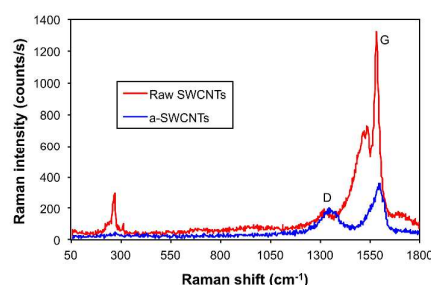
Fig. 2. Raman spectra of raw SWCNTs and a-SWCNTs.
