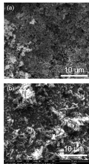
Fig. 12. SEM images of copper (a) anode and (b) cathode surfaces after electrolysis of a suspension of a-SWCNTs (0.0034 mg/mL) in a solution of acetic acid ( 0.85 \text{ mol/dm}^3 ). Scale bars = 10 \mu\text{m} .
