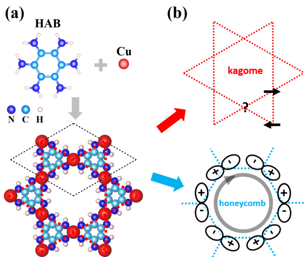
Fig. 1 Structural and electronic properties of \text{Cu}_3(\text{HAB})_2 . (a) Atomic structure of a HAB molecule and the crystalline structure of \text{Cu}_3(\text{HAB})_2 by coordinating HAB with Cu. (b) Schematics of two frustrations in this material.
