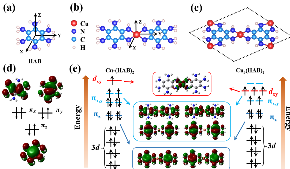
Fig. 3 Molecular information. (a) HAB molecule. (b) Cu-(HAB) 2 complex. (c) Cu 3 (HAB) 2 crystal. (d) Wavefunctions of HAB molecule. (e) Energy levels and the associated wavefunctions of (b) a Cu-(HAB) 2 complex (left) and (c) Cu 3 (HAB) 2 crystal (right).
