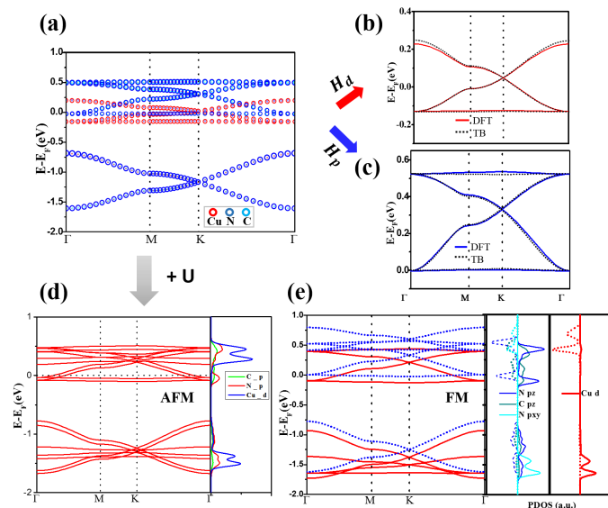
Fig. 2 Band structures from DFT, DFT+U and the effective TB models. (a) Atomic-resolved DFT band structure; the marker size indicates the weight of the atomic composition. Decomposition of the bands into (b) a kagome lattice and (c) a honeycomb lattice, with comparison to the effective TB model band structure. (d) The DFT+U AFM band structure and the projected density of states (PDOS). (e) The DFT+U FM band structure and PDOS. The solid and dashed curves correspond to different spins.
