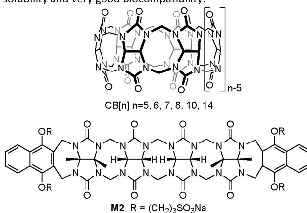
Figure 1 Chemical structures of CB[n] and the prototypical acyclic CB[n]-type molecular container M2 .
