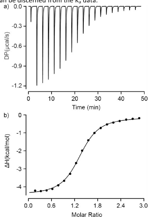
Figure 6 a) ITC thermogram recorded during the titration of receptor 1 (100 \mu M) in the cell with guest 11 (1.5 mM) in the syringe, b) Fitting of the data to a 1:1 binding model with K_a = (2.28 \pm 0.3) \times 10^5 \text{ M}^{-1} .
