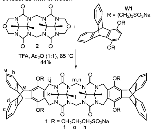
Figure 2 Synthesis of host 1 .
