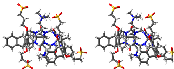
Figure 7 Cross eyed stereoview of an MMFF minimized model of the 1•12 complex. Color code: C, grey; H, white; N, blue; O, red.
