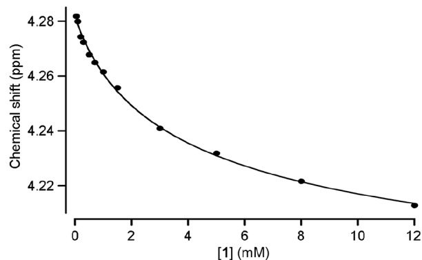
Figure 4 Plot of chemical shift of H n versus [1] used to determine the self-association constant K s = 507 ± 62 M -1 for 1 .
