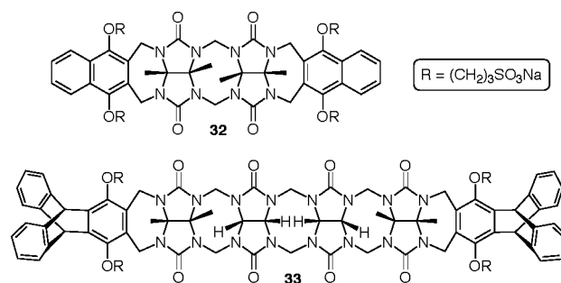
Figure 8 Chemical structures of comparison hosts 32 and 33 .
