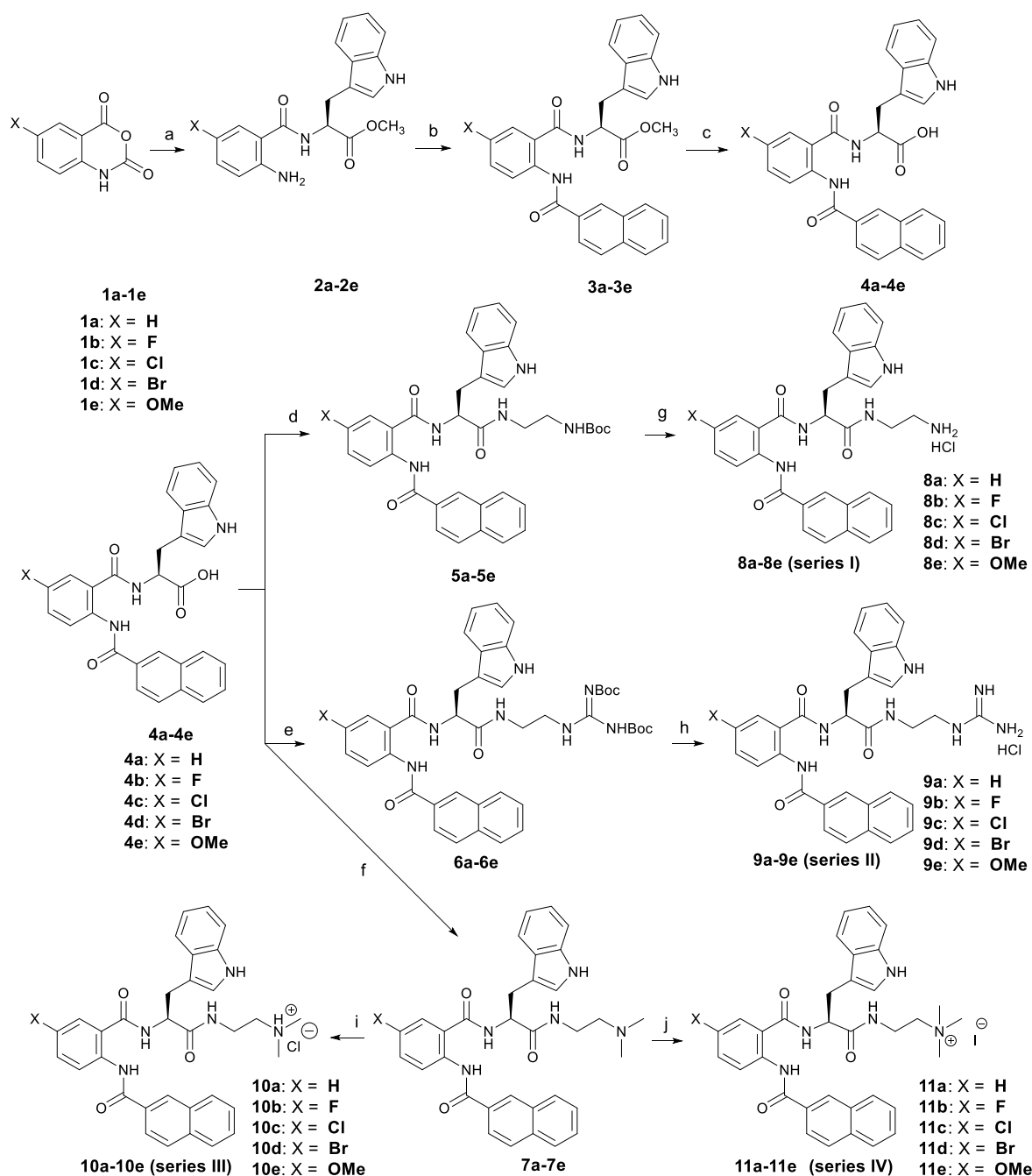
Scheme 1 General synthetic scheme to synthesize anthranilic acid-based peptidomimetics. Reaction conditions: a) isatoic anhydrides (1.0 equiv), methyl- L -tryptophanate (1.0 equiv), CH 3 CN, reflux, 16 h; b) 2-naphthoyl chloride (1.0 equiv), Et 3 N (3.0 equiv), CH 2 Cl 2 , rt, 4 h; c) 1 N NaOH (aq) (2.0 equiv), THF, MeOH, rt, overnight; d) N -Boc-1,2-diaminoethane, EDCI (1.2 equiv), HOBT (1.0 equiv), DIEA (2.5 equiv), DMF, rt, overnight; e) 1-(2-aminoethyl) 2,3-bis( tert -butoxycarbonyl)guanidine, EDCI (1.2 equiv), HOBT (1.0 equiv), DIEA (2.5 equiv), DMF, rt, overnight; f) N,N -dimethylethylenediamine, EDCI (1.2 equiv), HOBT (1.0 equiv), DIEA (2.5 equiv), DMF, rt, overnight; g) 4 N HCl in dioxane, CH 2 Cl 2 , rt, 4 h; h) TFA, CH 2 Cl 2 , rt, 8 h; 4 N HCl in dioxane, CH 2 Cl 2 , rt, 30 min; i) 4 N HCl in dioxane, CH 2 Cl 2 , rt, 30 min; j) CH 3 I (2.0 equiv), CH 3 CN, rt, overnight.
