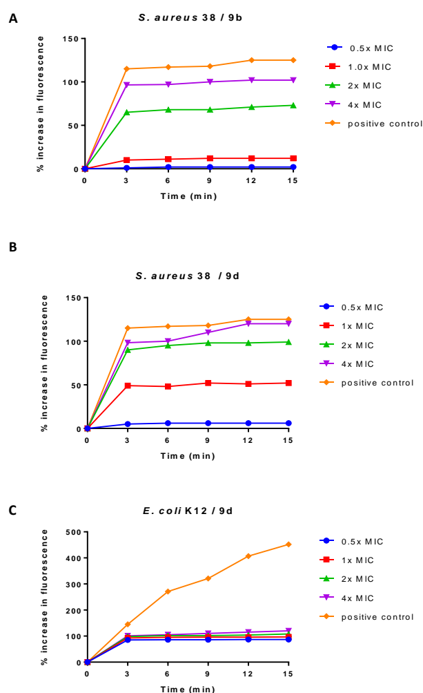
Fig. 3. S. aureus cytoplasmic membrane disruption promoted by (A) 9b (1.0 \mu\text{M} , 2.0 \mu\text{M} , 4.0 \mu\text{M} , 8.0 \mu\text{M} ) and (B) 9d (1.95 \mu\text{M} , 3.9 \mu\text{M} , 7.8 \mu\text{M} , 15.6 \mu\text{M} ) at different concentrations. (C) E. coli cytoplasmic membrane disruption promoted by 9d (7.8 \mu\text{M} , 15.6 \mu\text{M} , 31.2 \mu\text{M} , 62.4 \mu\text{M} ) at different concentrations. 20% DMSO was used as positive control.
