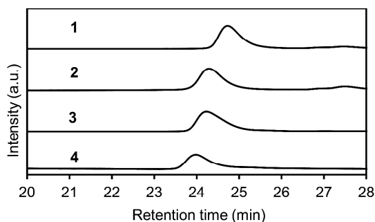
Fig. 4. Elution profiles of hybrids (a) 1 , (b) 2 , (c) 3 , and (d) 4 from GPC in THF (1 mL/min; 40 °C).
