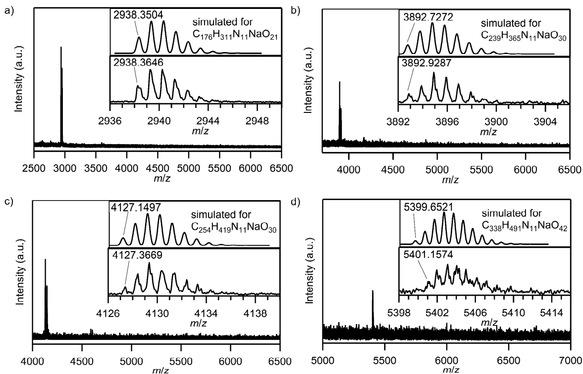
Fig. 3. MALDI-TOF mass spectra of peptide-dendron hybrids (a) 1 , (b) 2 , (c) 3 , and (d) 4 . The inset compares the simulated isotope pattern 61 (upper) with the observed isotope distribution (lower) for the [M + Na]^+ ion.
