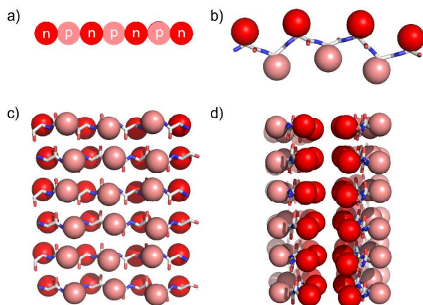
Fig. 2. (a) Pattern of non-polar (n, red color) and polar (p, pink color) amino acids employed in the design of \beta -sheet-forming peptides. (b) Schematic model of a peptide in the extended \beta -strand conformation with colored spheres indicating the relative orientation of the side chains. (c) Schematic model of an antiparallel \beta -sheet assembly of the peptide designed by hydrophobic patterning. (d) Packing of the non-polar faces of two \beta -sheet assemblies.
