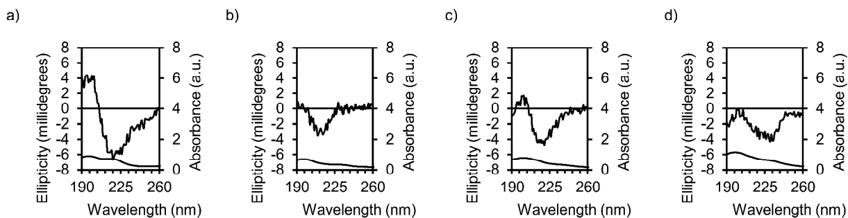
Fig. 7. Circular dichroism spectra (upper curve, left-hand axis) and UV–vis spectra (lower curve, right-hand axis) from films of (a) 1 , (b) 2 , (c) 3 , and (d) 4 on quartz. Spectra were recorded at 20 °C.
