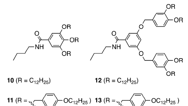
Fig. 6. Structures of the dendritic butyl amides 10–13 .
