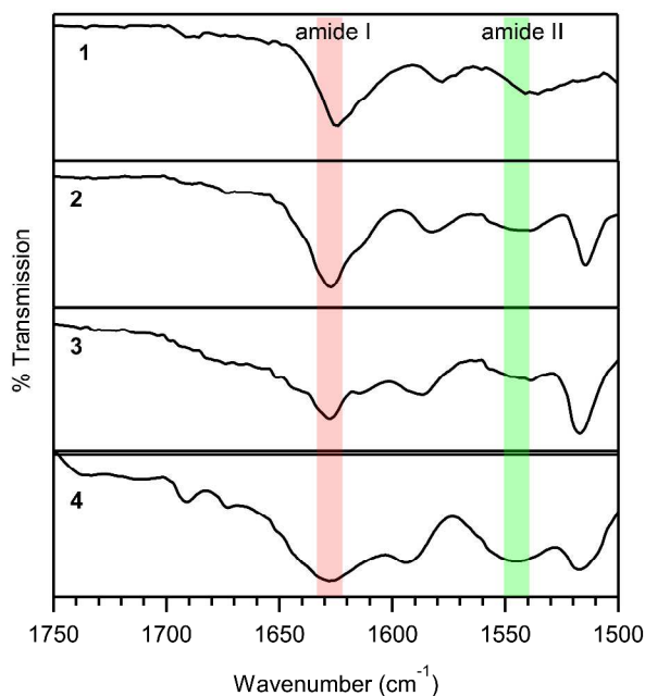
Fig. 5. Infrared spectra of peptide-dendron hybrids 1–4 acquired at room temperature from spin-cast films.
