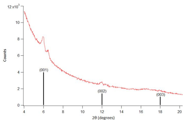
Figure 4: Measured data (red, top) (Cu K \alpha 1.5418 Å) and line representation of published XRD data (black, bottom) for out of plane reflection for tetragonal P4 structure identified for Cu(bpdc) in 14 . The set of larger peaks in the experimental data matched the literature patterns. The set of small peaks is due to the formation of a second crystalline structure which appeared after several hours of XRD data collection.
