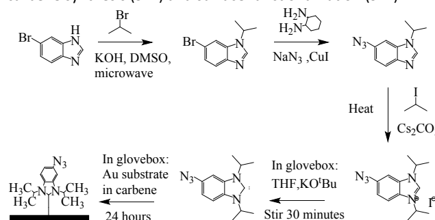
Figure 2. Scheme for Au-carbene SAM synthesis modified from the literature. 25
