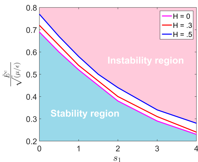
Fig. 7 Stability and instability regions in the dead load ( s_1 ) - electric field plane of a neo-Hookean dielectric film under various magnetic fields H = 0, 0.3, 0.5 . The stability region is enclosed by the curve of zero determinant and the axes. A higher magnetic field corresponds to a larger stability region.
