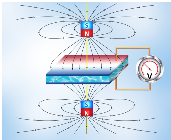
Fig. 1 Schematic figure illustrating the mechanism that can be used to engineer the magneto-electric effect in soft materials. A thin film made of an elastically soft material is coated with two compliant electrodes. When subjected to a pre-existing electric potential, the dielectric will be deformed and be polarized by the electric field. Now, if an external magnetic field is switched on, the magnetic Maxwell stress will also deform the thin film if its magnetic permeability \mu_r > 1 . That, in turn, alters the existing polarization and deformation. The change of the polarization in the film can be measured as a current due to the imposed magnetic field and thus manifests as an emergent strain-mediated magneto-electric effect.
