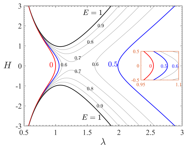
Fig. 6 Behavior of a neo-Hookean dielectric film at a zero dead load S = 0 under various nominal electric field from E = 0 to E = 1 in equilibrium: in-plane stretch \lambda vs. magnetic field H .
