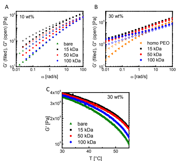
Fig. 2 Frequency sweeps of 100 kDa PEO homopolymer and its composites loaded with 15 kDa, 50 kDa, 100 kDa PVAc-adsorbed and bare particles at 85°C for (A) 10 wt% and (B) 30 wt% loadings. (C) Effect of adsorbed chain length on elastic modulus is observed in temperature sweeps at 1% strain and 5rad/s frequency for 30 wt% loading.
