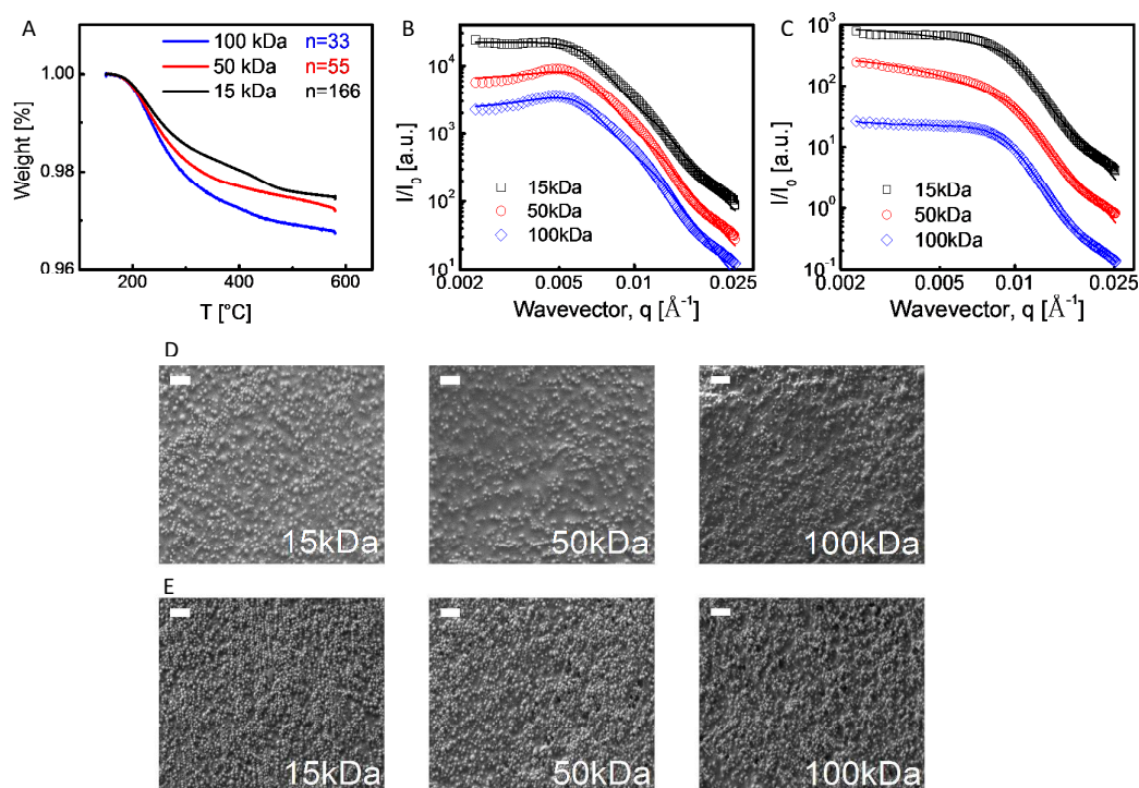
Fig. 1 (A) TGA data of PVAc with varying molecular weights adsorbed on silica nanoparticles is used to determine the number of adsorbed chains on particles ( n ). SAXS profiles of PEO nanocomposites with (B) 10 wt% and (C) 30 wt% silica nanoparticles adsorbed with PVAc of varying molecular weights 15 kDa, 50 kDa and 100 kDa. Lines represent the model fits. SEMs of 15 kDa, 50 kDa and 100 kDa PVAc adsorbed particles in 100 kDa PEO matrices. Data is for composites with (D) 10 wt% and (E) 30 wt% particle loading. Scale bar is 500 nm.
