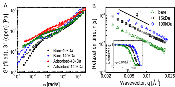
Fig. 5 (A) Effect of matrix molecular weight on the viscoelastic properties of PMA composites at a reference temperature of 55°C. Molecular weights in the labels are for the matrix. Molecular weight of adsorbed PVAc is 50 kDa. (B) Relaxation times of 15 kDa and 100 kDa PVAc-adsorbed and bare nanoparticles in 140 kDa PMA matrix. Data is collected at 160°C. The inset shows intensity autocorrelation function at q=0.010 \text{ \AA}^{-1} . Particle loading is 30 wt% in all samples.
