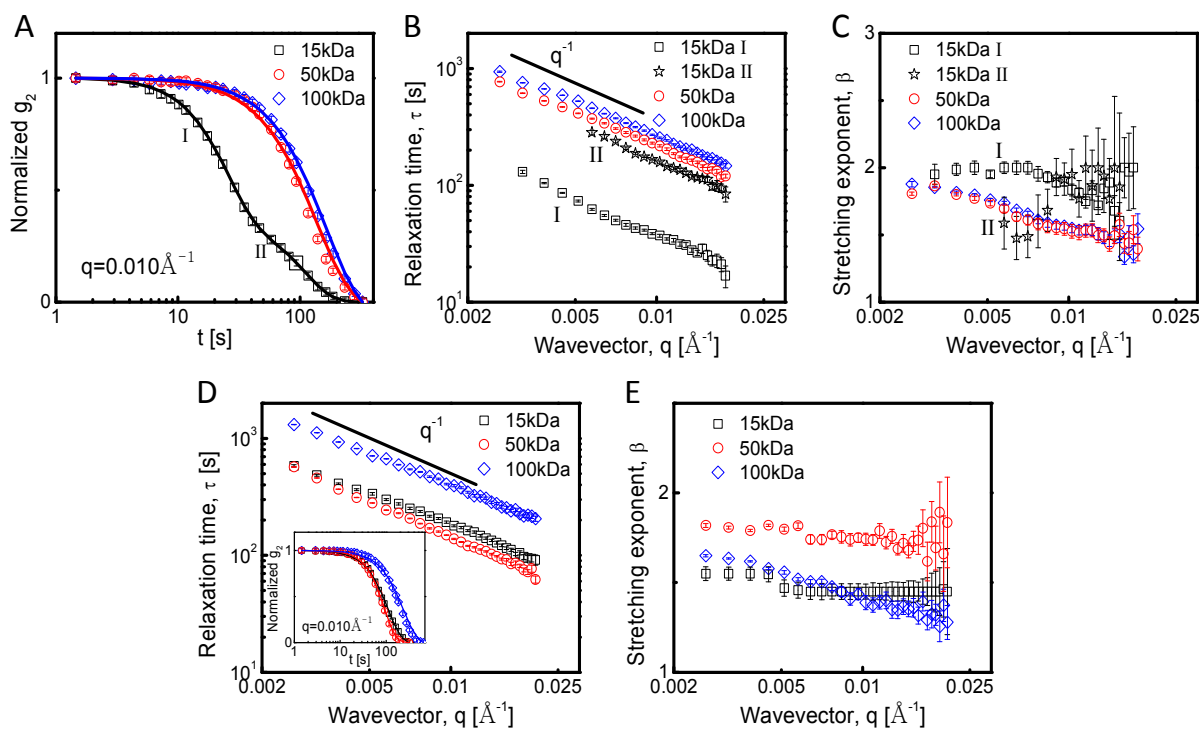
Fig. 3 Effect of adsorbed PVAc chain lengths (15 kDa, 50 kDa, 100 kDa) on nanoparticle dynamics: (A) autocorrelation function at q=0.01 \text{ \AA}^{-1} , (B) relaxations times and (C) stretching exponent as a function of scattering vector, q . Samples are composites of 100 kDa PEO with 10 wt% loading. Data is collected at 80^\circ\text{C} . 15 kDa sample has two different decay rates which are labeled as I and II in (A) and relaxation times for the corresponding regions are shown in (B). (D-E) Relaxations and stretching exponent of particles adsorbed with PVAc of different chain lengths in 100 kDa PEO at 80^\circ\text{C} with 30 wt% loading. Inset in (D) shows the intensity autocorrelation function at q=0.010 \text{ \AA}^{-1} .
