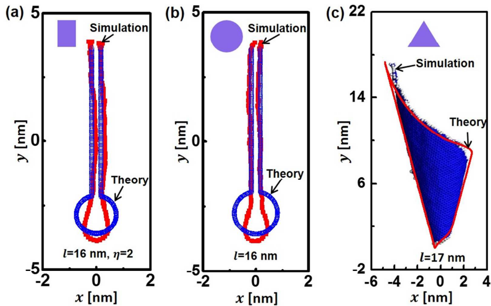
Figure 6. Comparison of overall configurations of self-folded graphene after complete evaporation of liquid between simulations and theoretical analysis. “Racket-like” pattern folded from planar (a) rectangular graphene with a length of l=16 nm, and (b) circular graphene with a length of l=16 nm. (c) “Cone-like” pattern folded from planar triangular graphene with a length of l=17 nm. Surface wettability of graphene in water \theta_c = 60^\circ .
