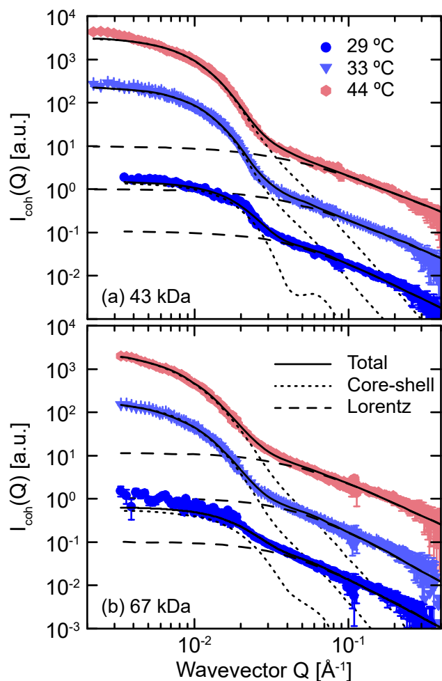
Fig. 3 Coherent scattering intensities I_{\text{coh}}(Q) for (a) 43 kDa and (b) 67 kDa polymer-grafted nanoparticles in d_{12} -cyclohexane at various temperatures. Solid curves are best fits to the sum of core-shell (dotted) and Lorentzian (dashed) form factors. Data and curves shifted vertically for clarity.
